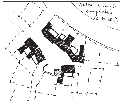
Step 25: the first street segment, completed
