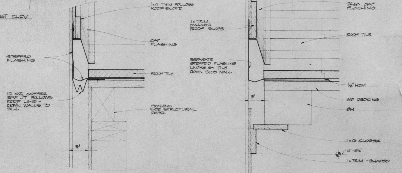
2 EXPANSION JT. B3 SCALE 3/4" = 1'-0"
