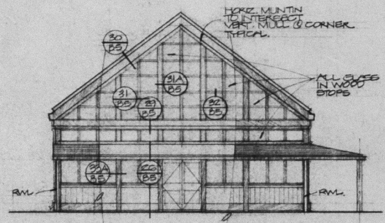
UNIT J WEST ELEV
