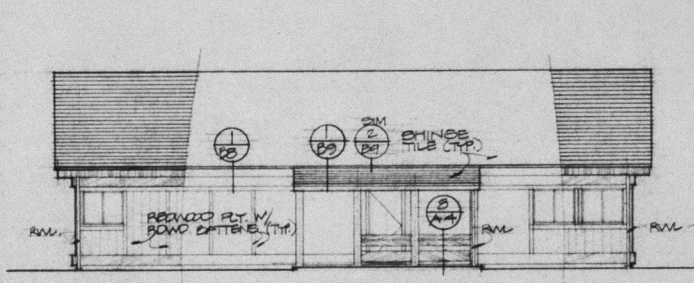
UNIT G NORTH ELEV
