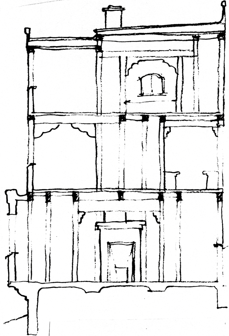
WINDOW SECTION
