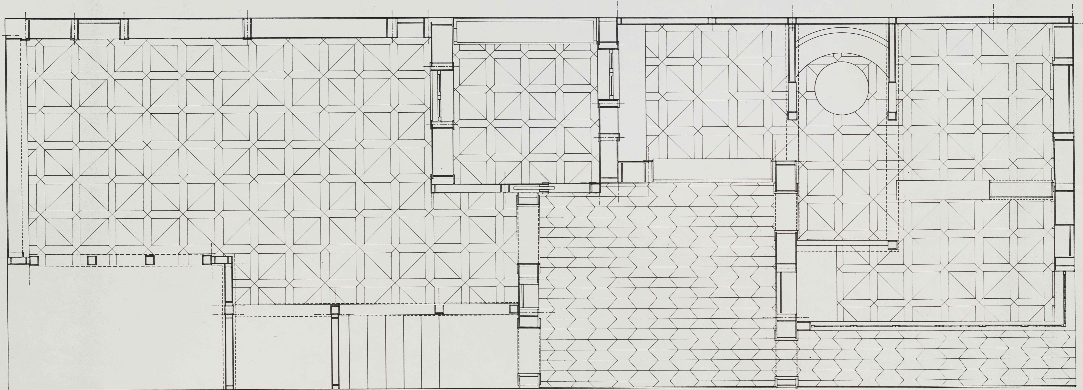
FLOOR PATTERNS 1" = 3/8"
