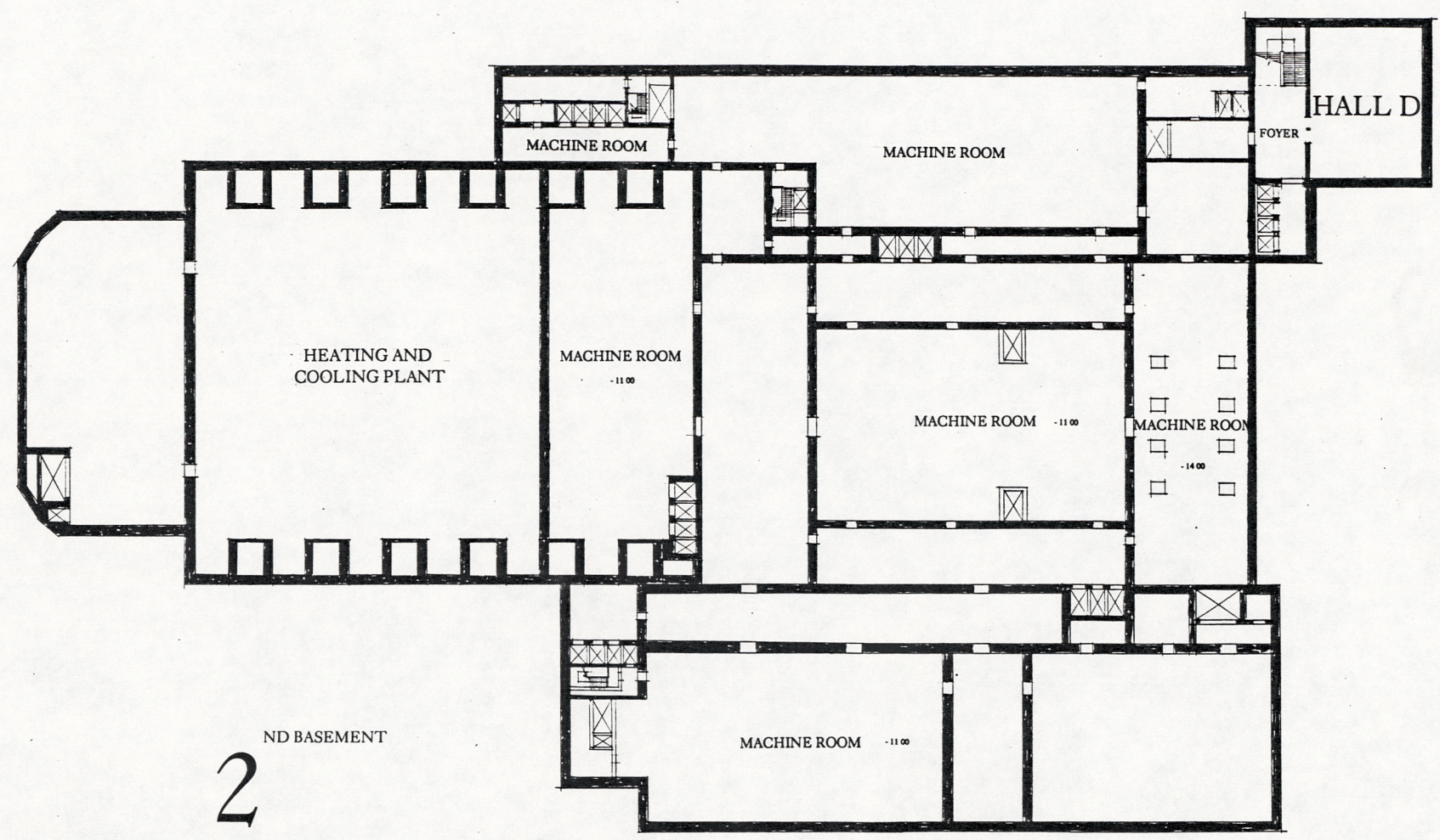
MINOR FLOOR: -11.00 and -14.00 meter levels
