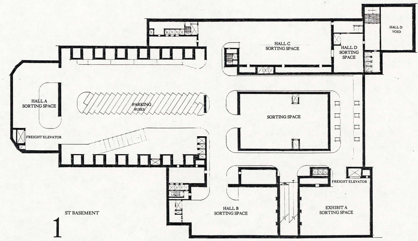
MINOR FLOOR: -5.50 meter level
