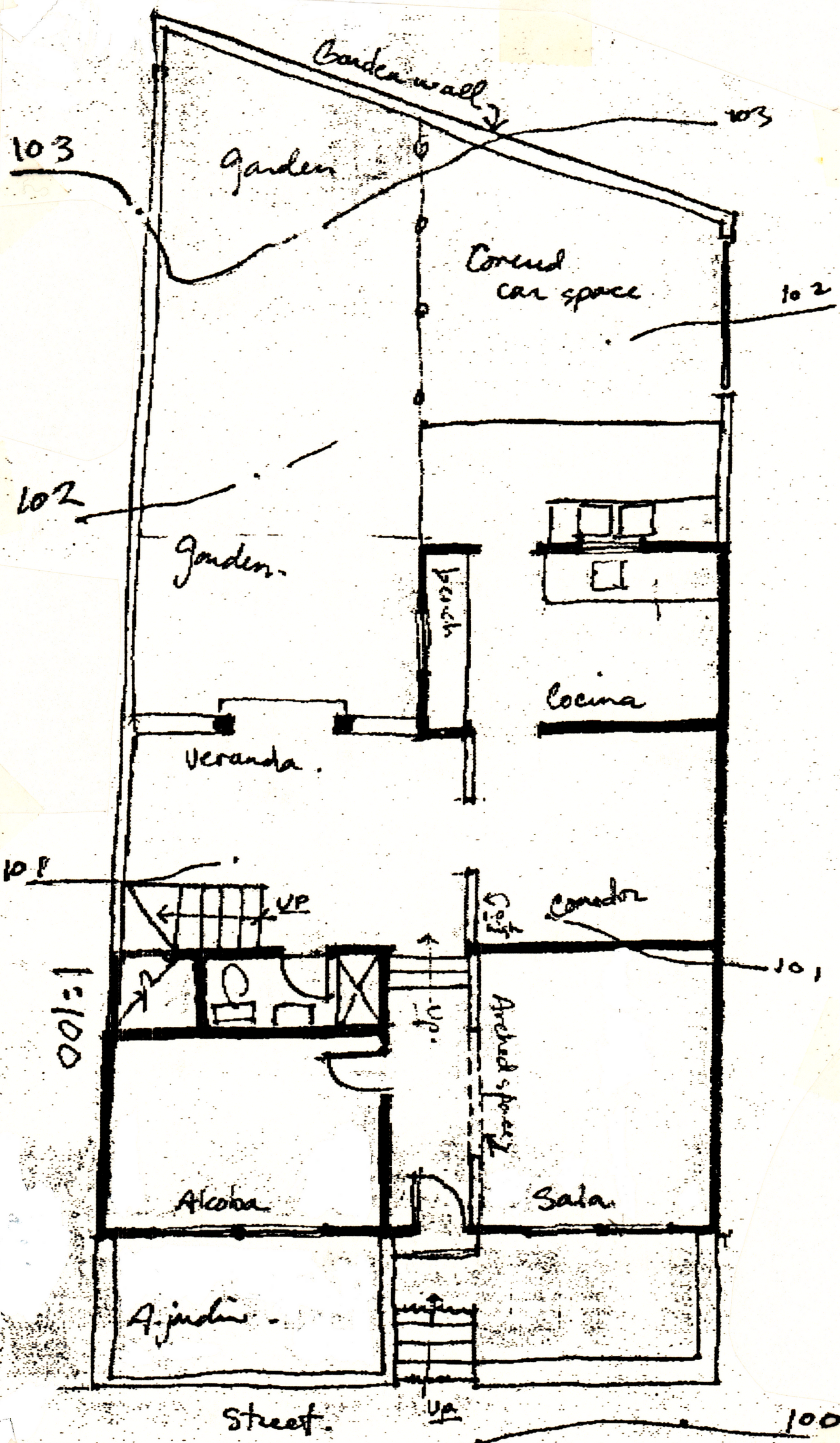
1ST FLOOR
