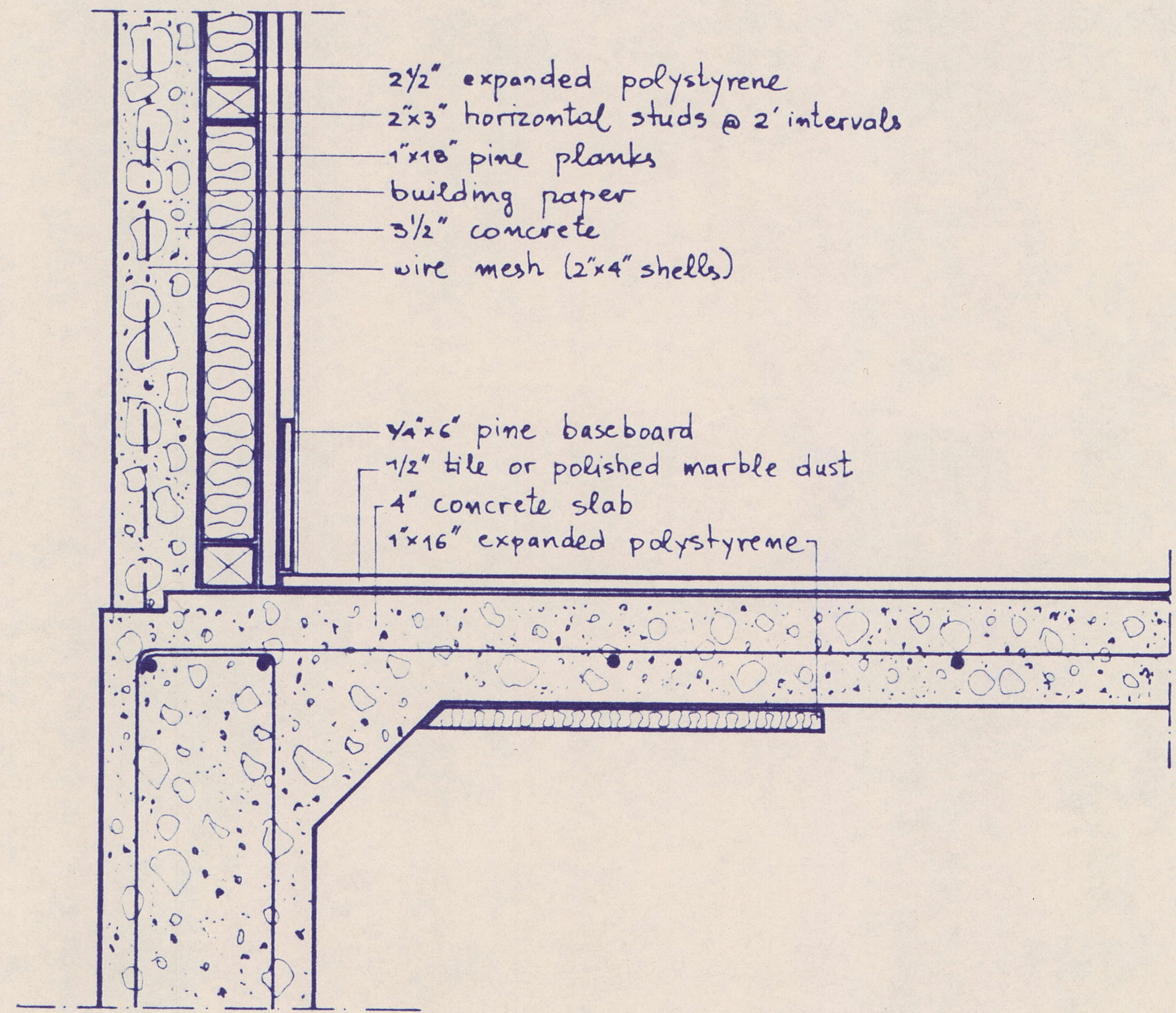
FLOOR AND TYPICAL WALL VERTICAL SECTION
