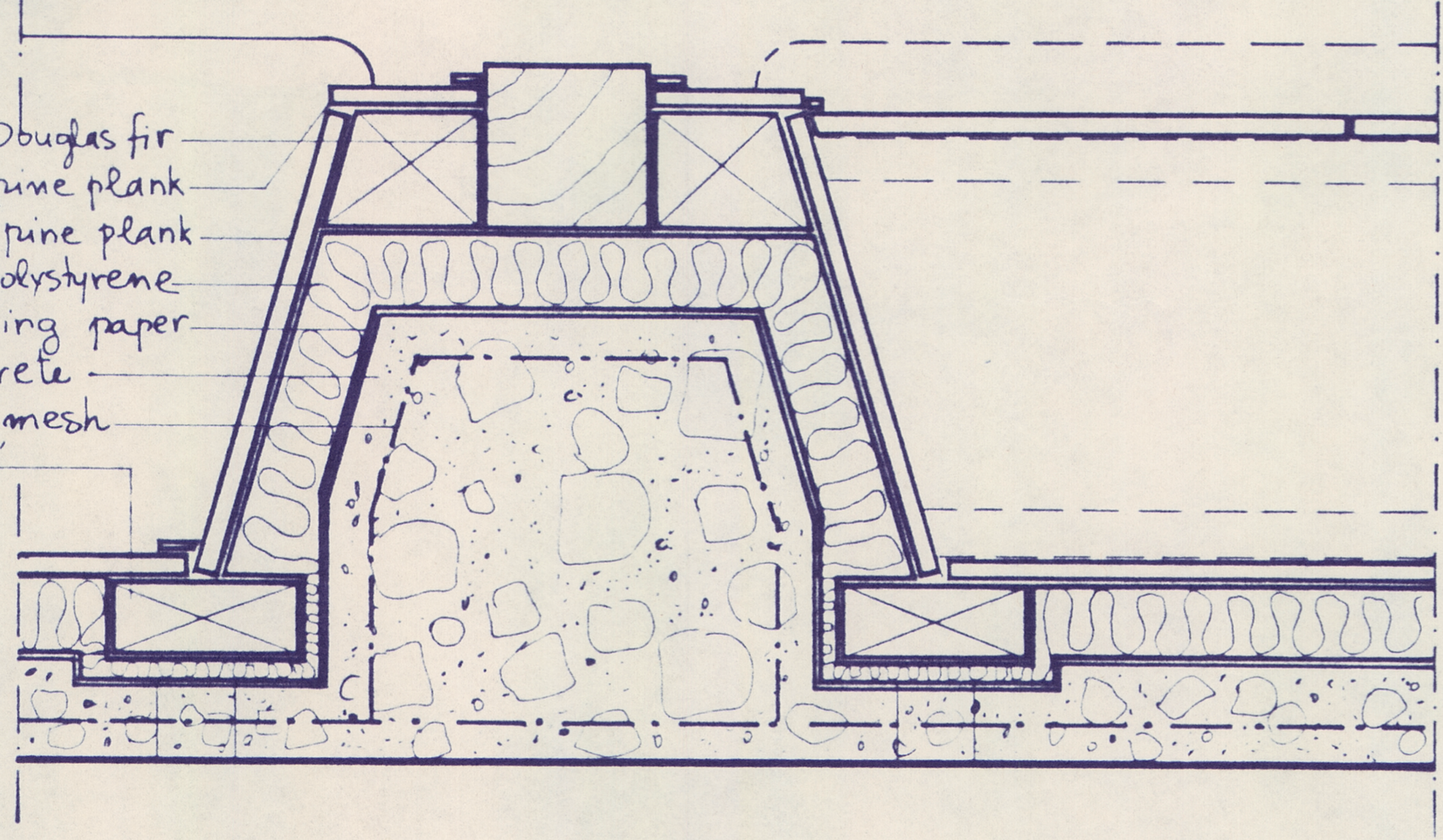
STUDIO WALL AND WINDOW SEAT - HORIZONTAL SECTION
