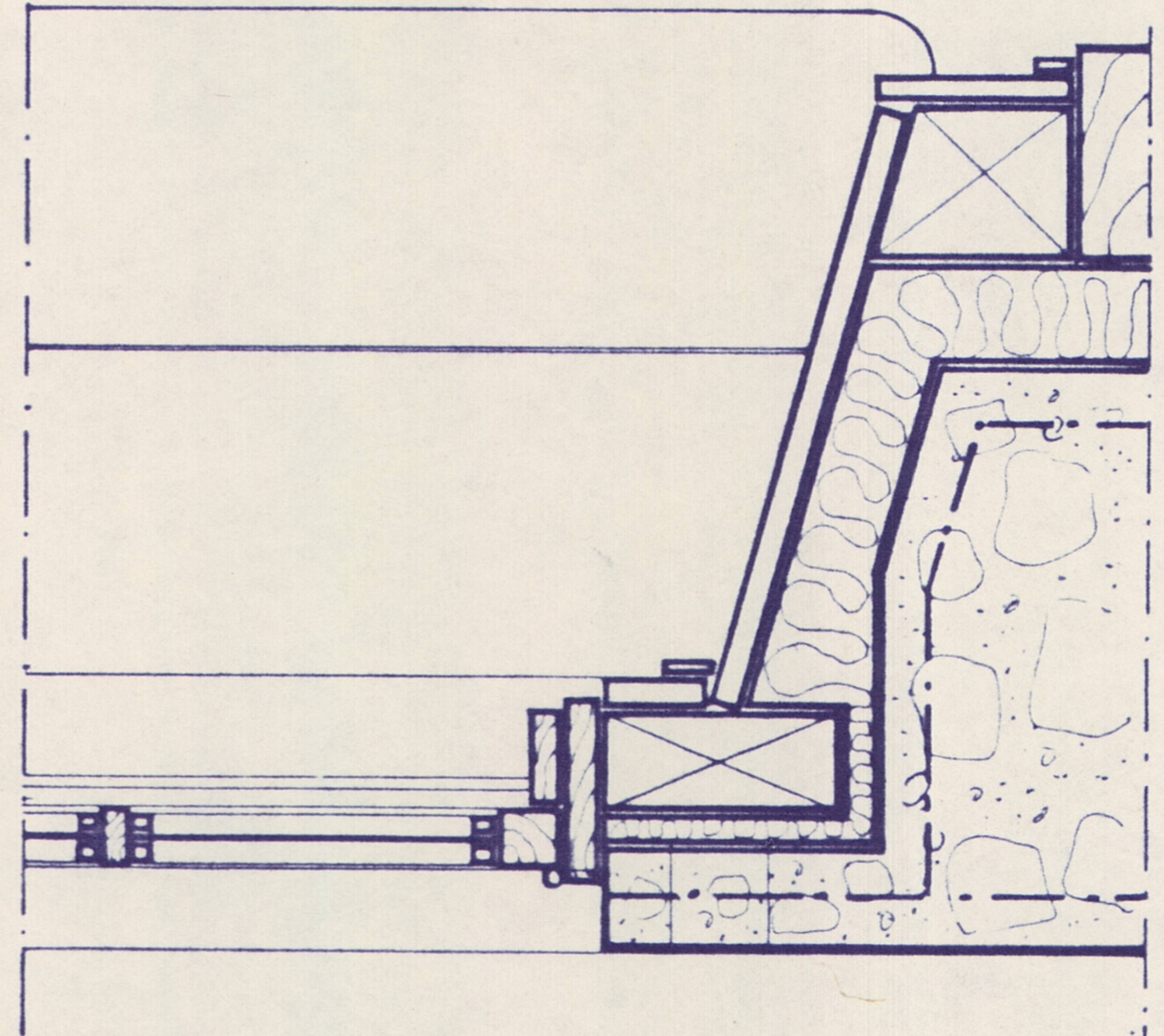
STUDIO WALL AND WINDOW SEAT - HORIZONTAL SECTION
