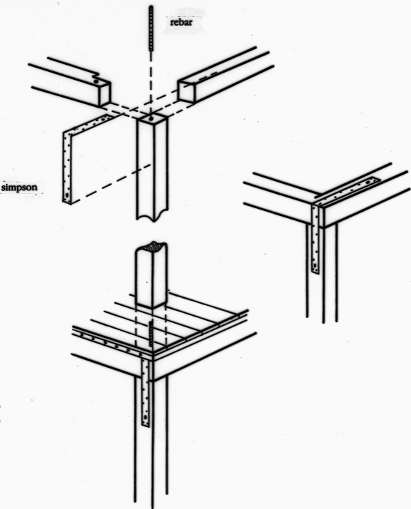
CORNER CONNECTIONS
