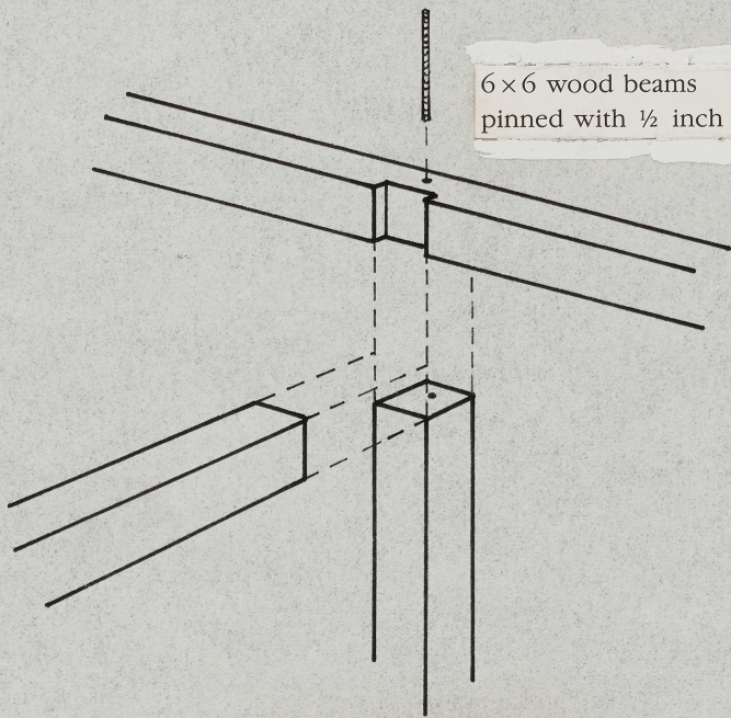
FRAMING CONNECTION
