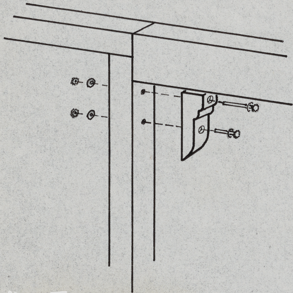
CORBEL cut from 6 × 6 fir
