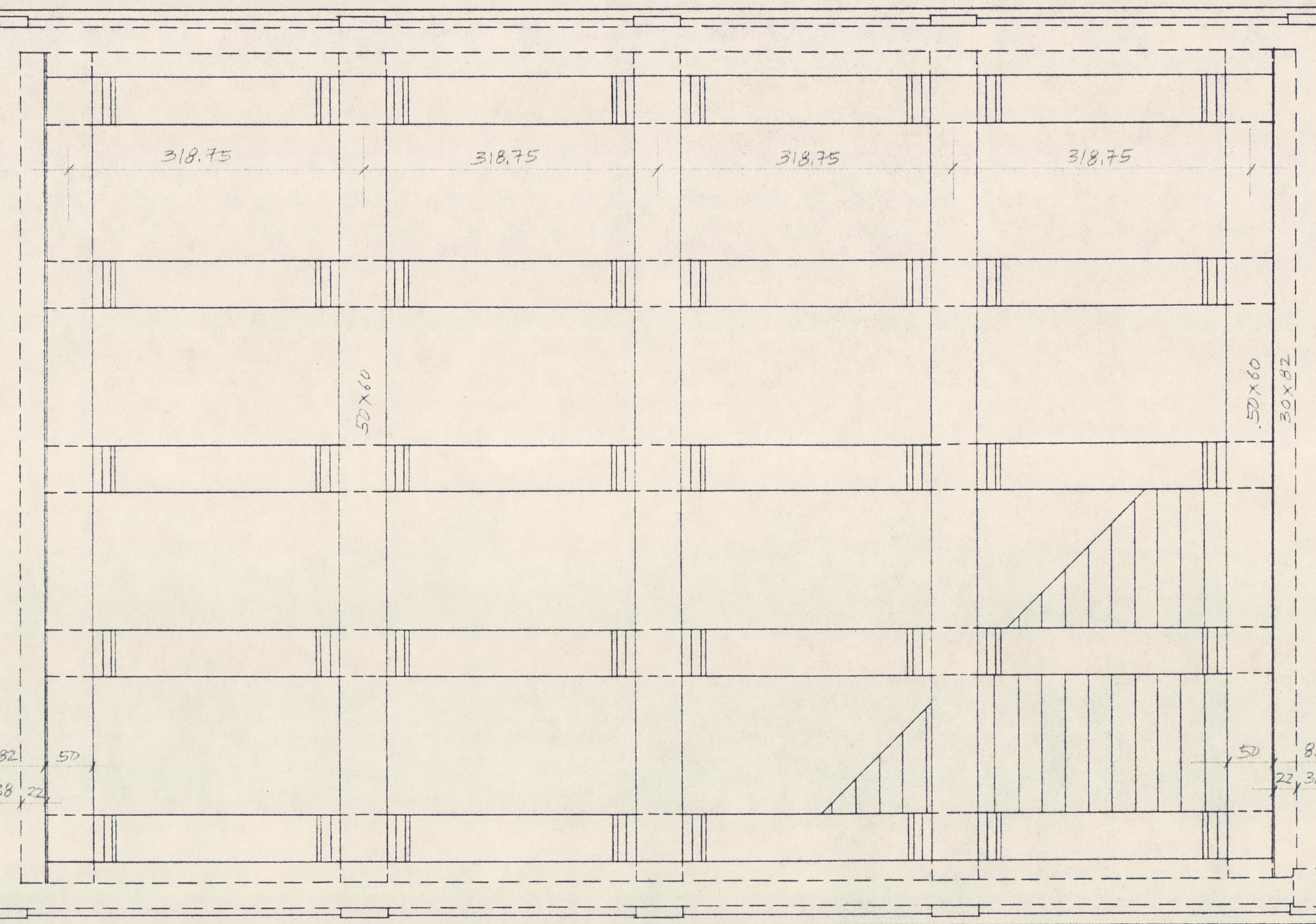
SECOND FLOOR FRAMING PLAN
