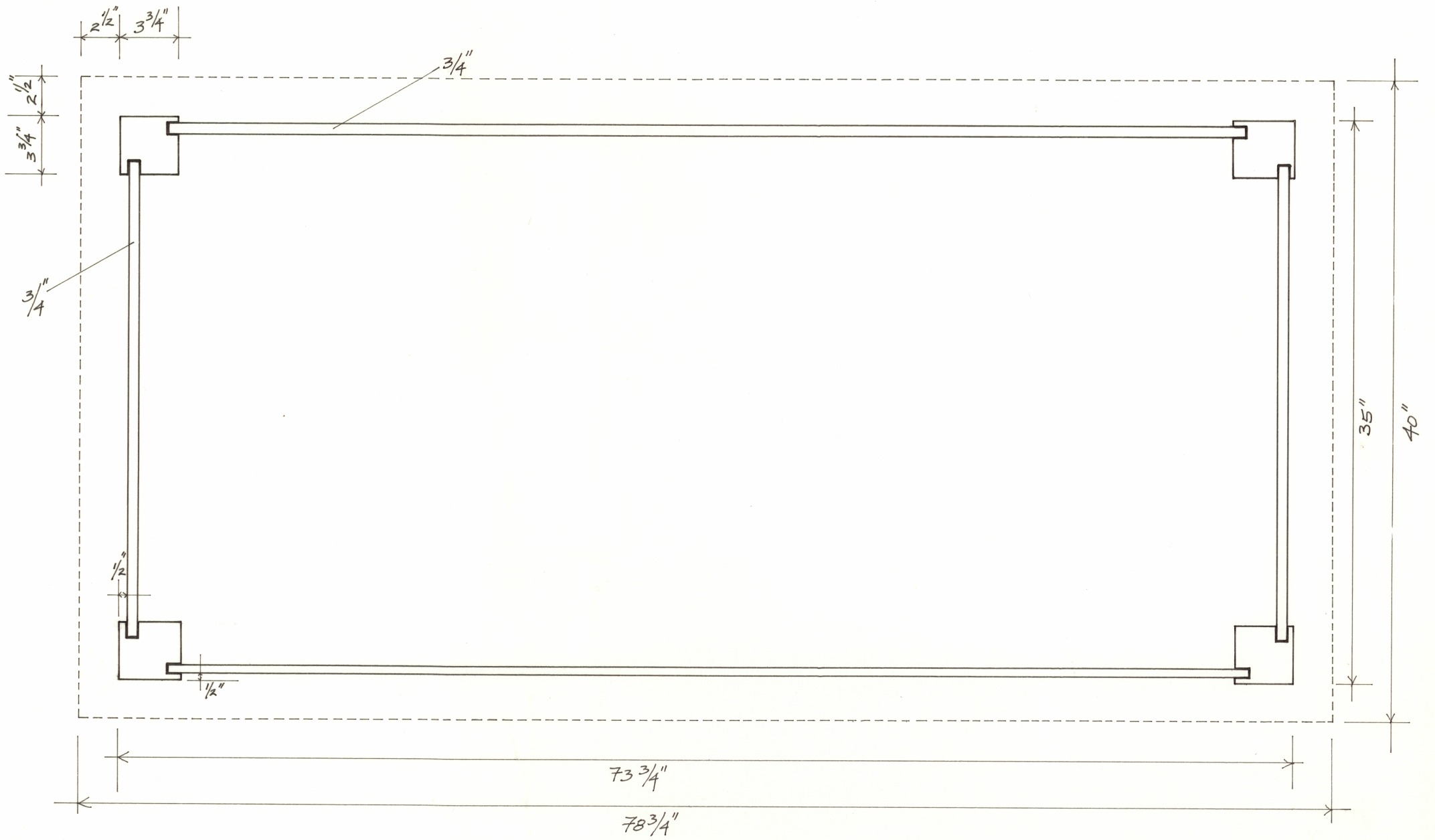
Horizontal Section 1' = 1/2''
