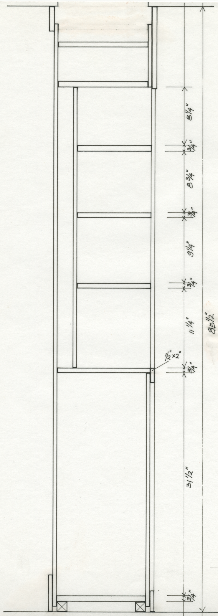
Vertical Section i=1\frac{1}{2}"
