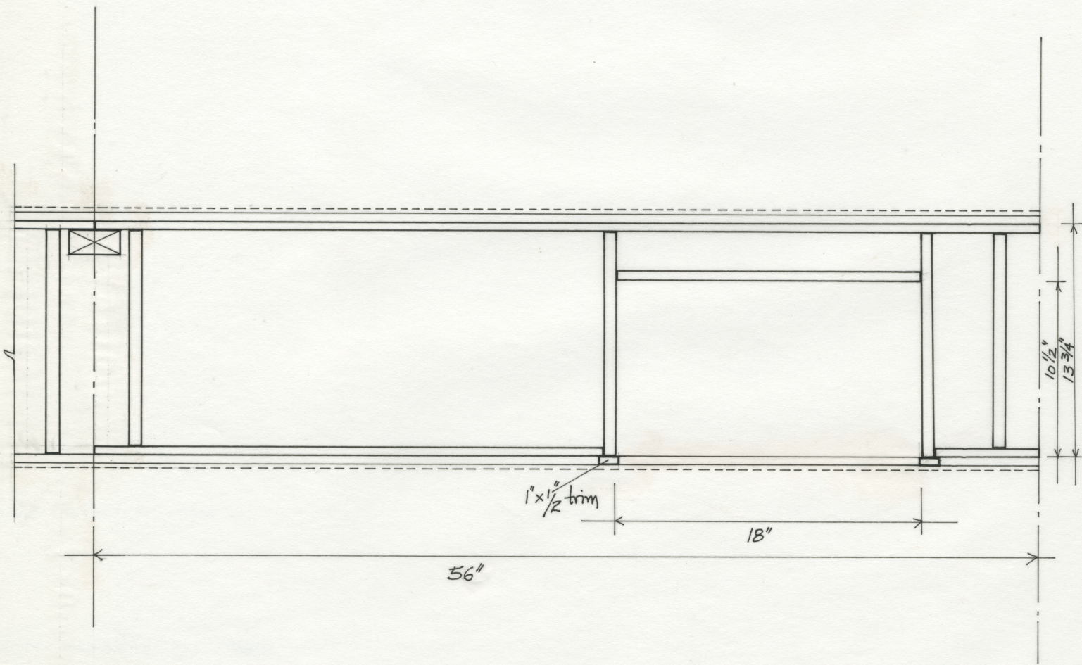
Horizontal Section 1" = 1 1/2"
