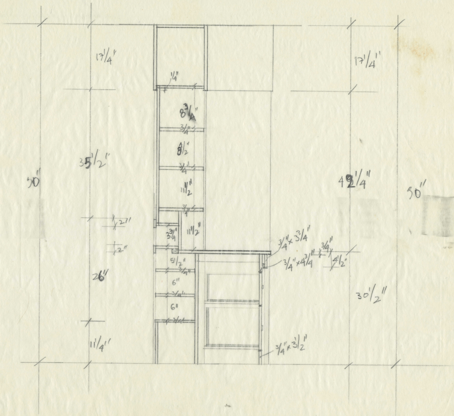
VERTICAL SECTION
