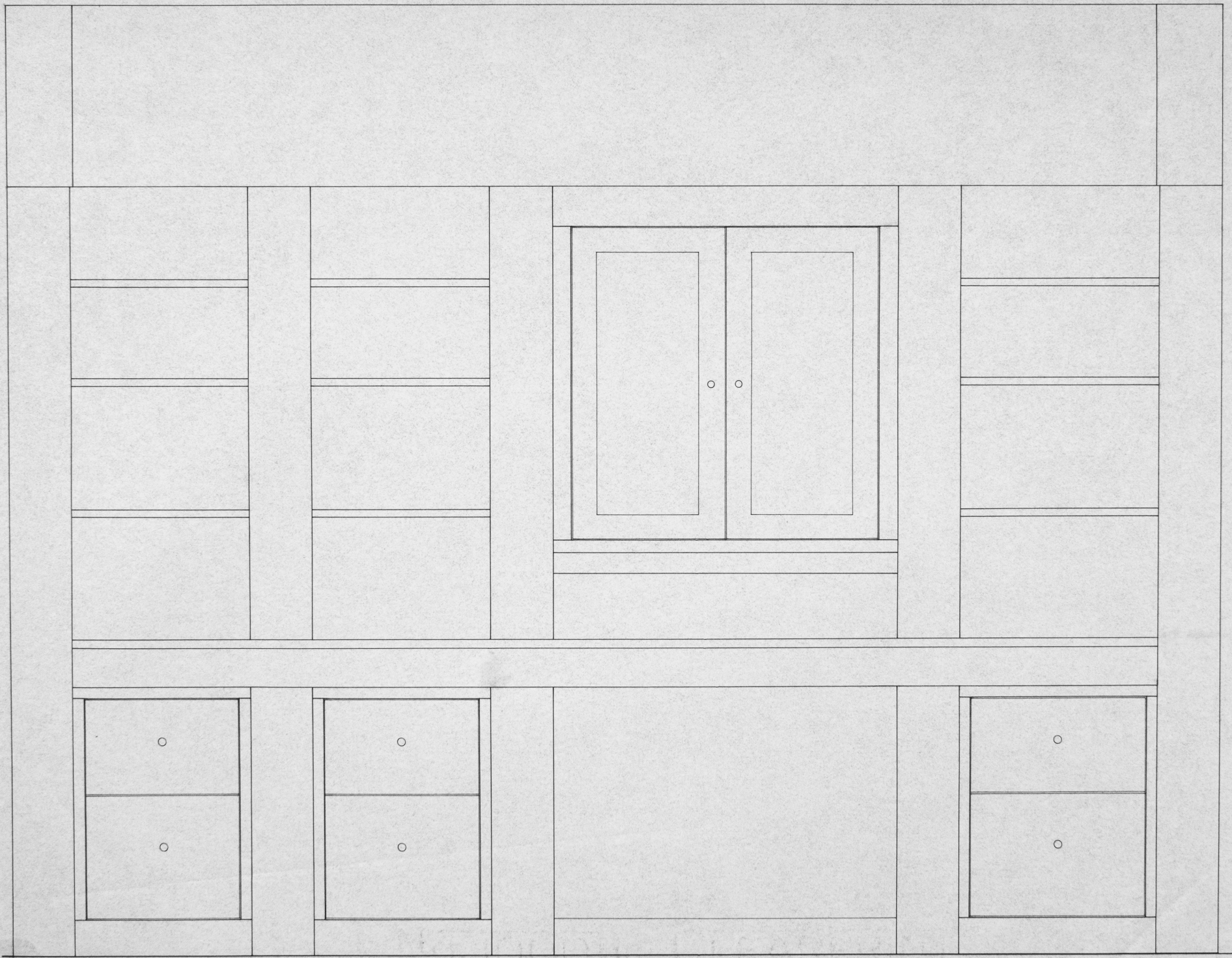
Front Elevation 1/2''
