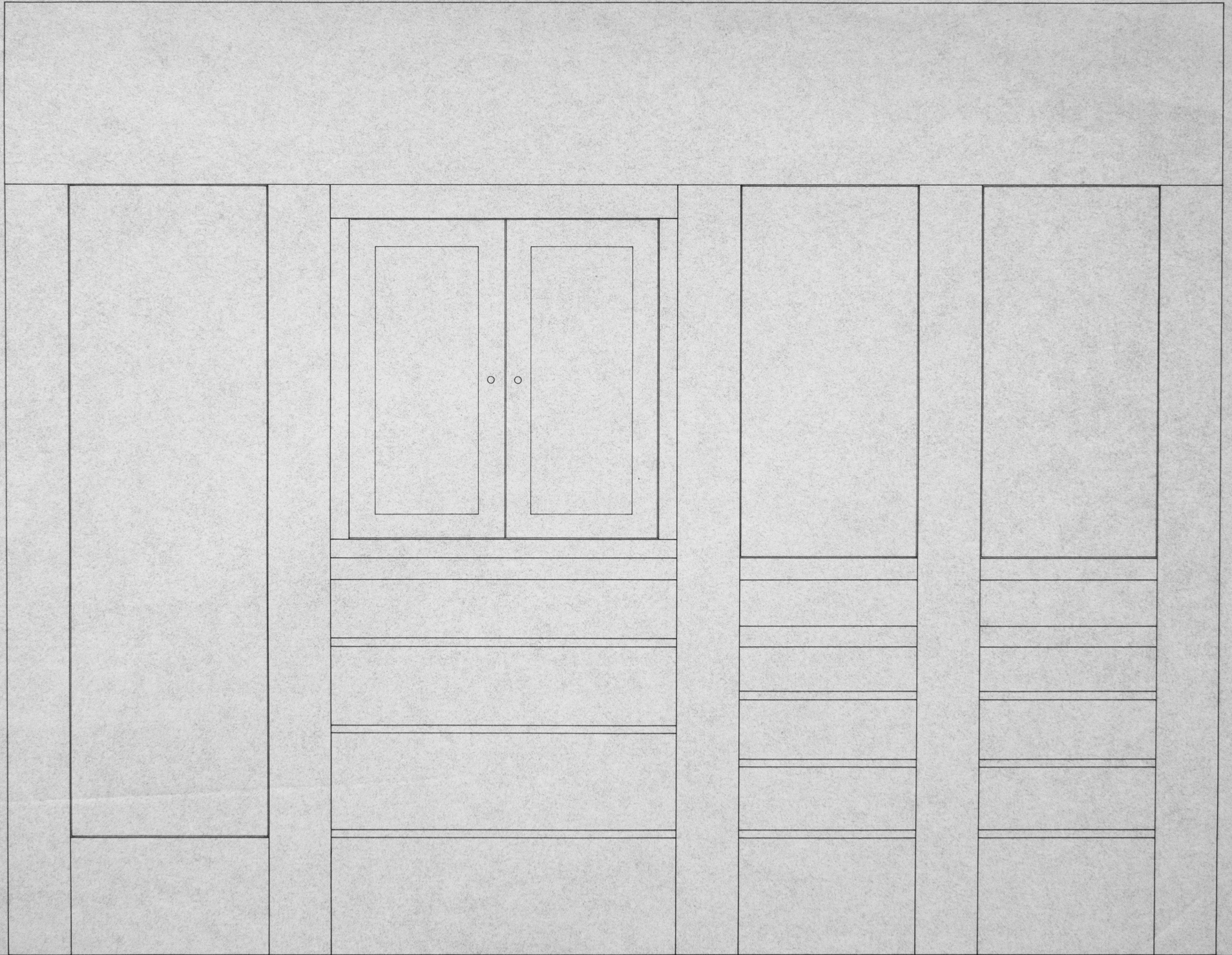
Back Elevation 1" = 1/2"
