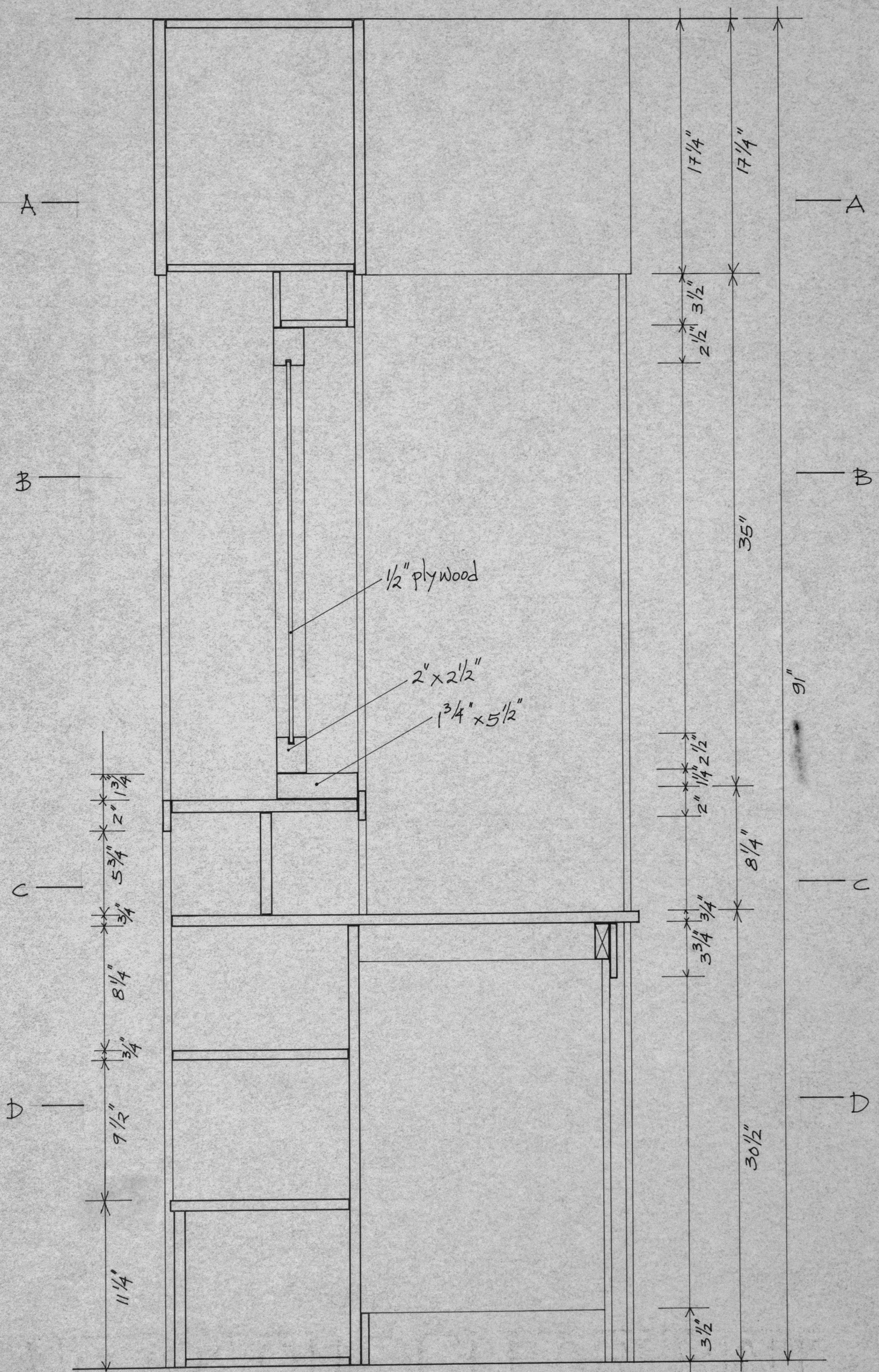
Vertical Section at window 1' = 1 1/2"
