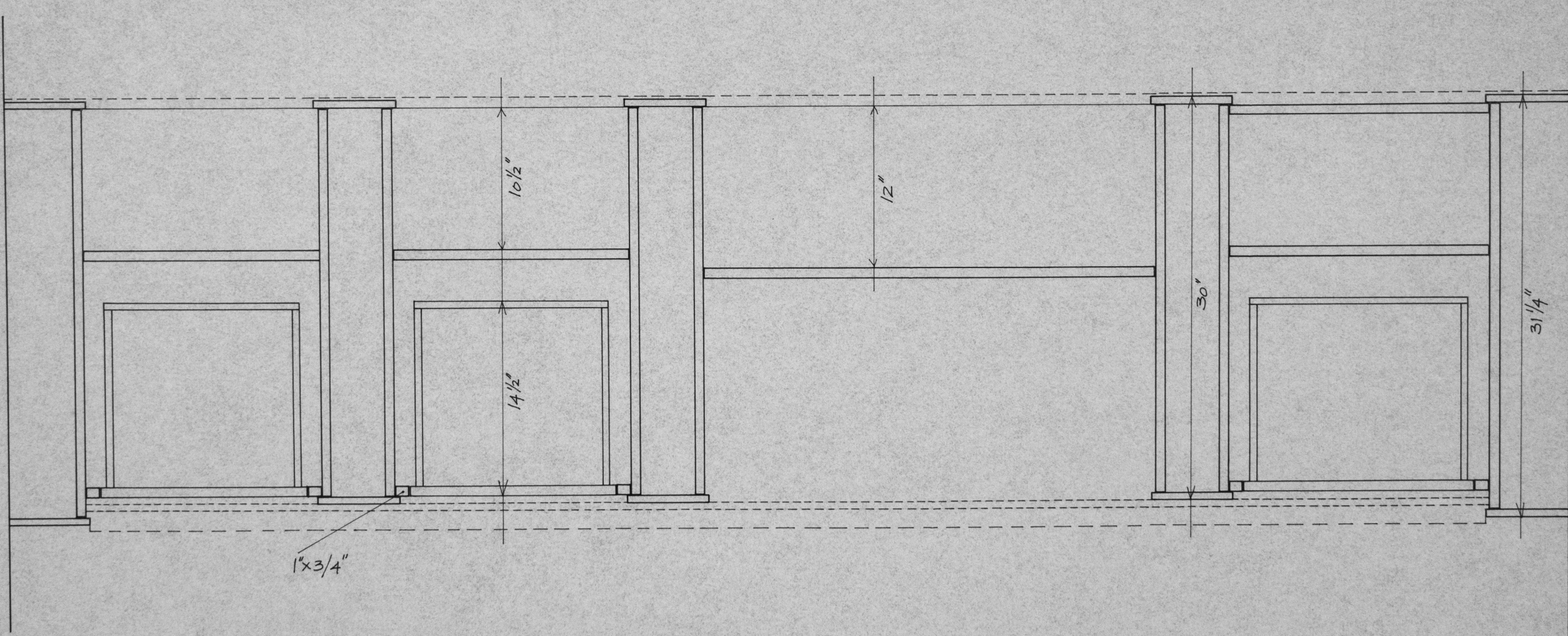
Horizontal Section D-D (below counter) 1' = \frac{1}{2}''
