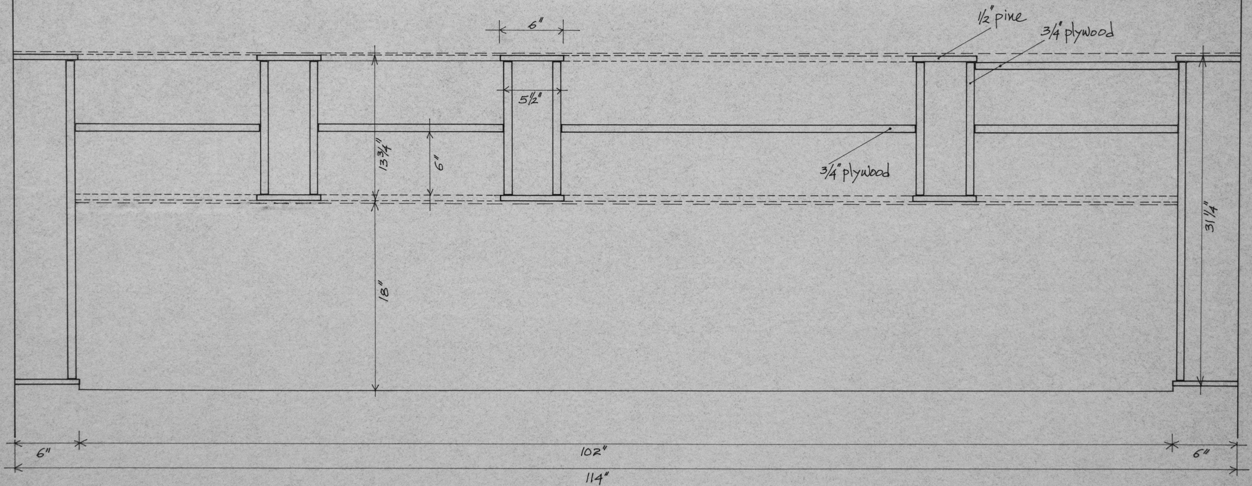
Horizontal Section c-c (above counter) 1' = 1 1/2"
