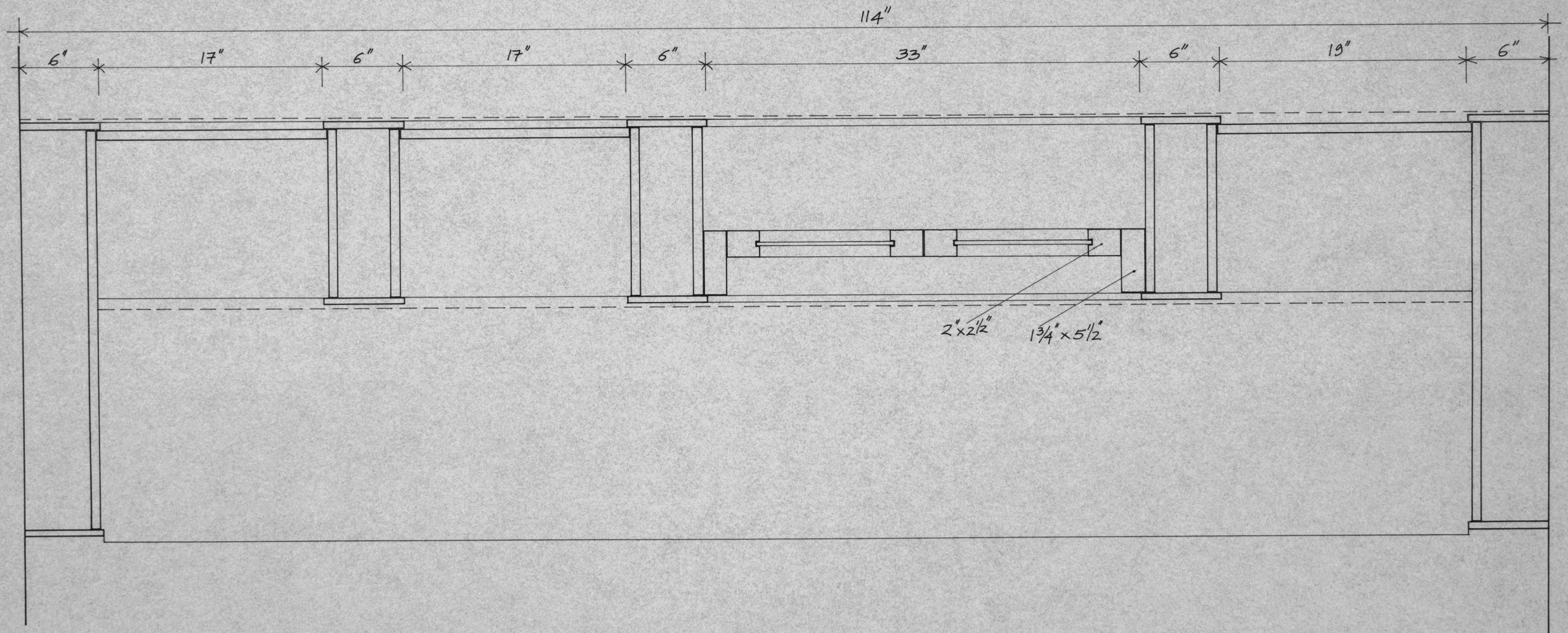
Horizontal Section B-B (at Window) 1' = 1\frac{1}{2}"
