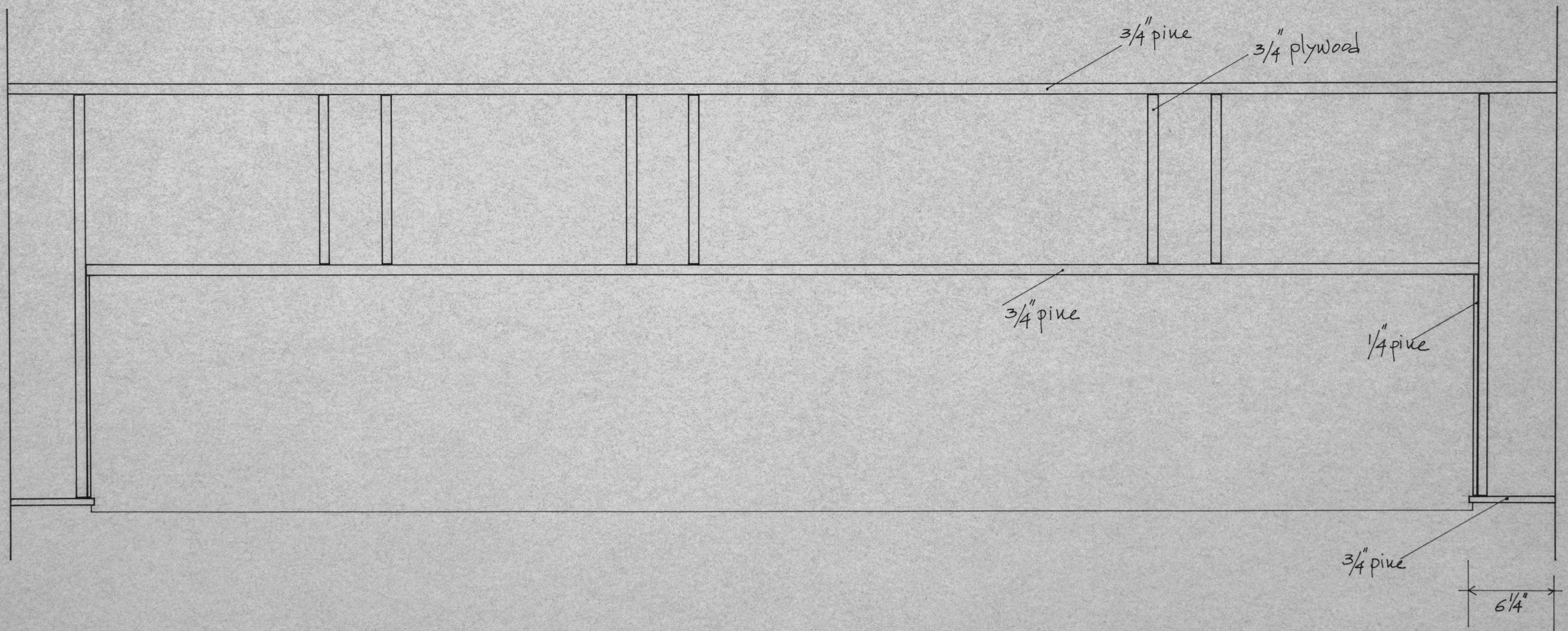
Horizontal Section at top 1' = 1 1/2" (Section A-A)
