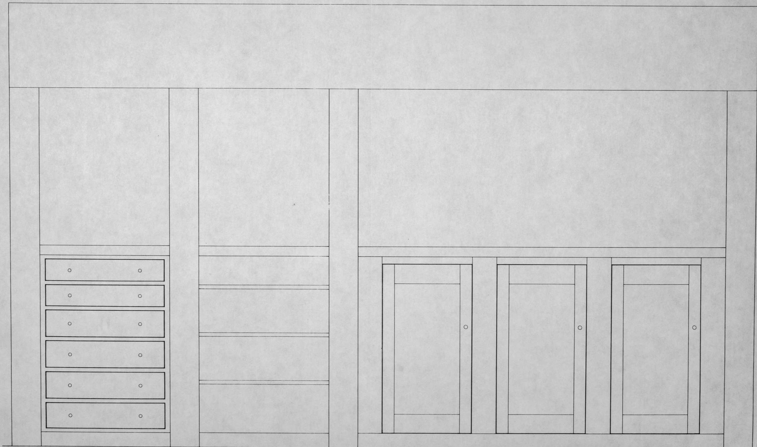
Elevation 1' = 1/2"
