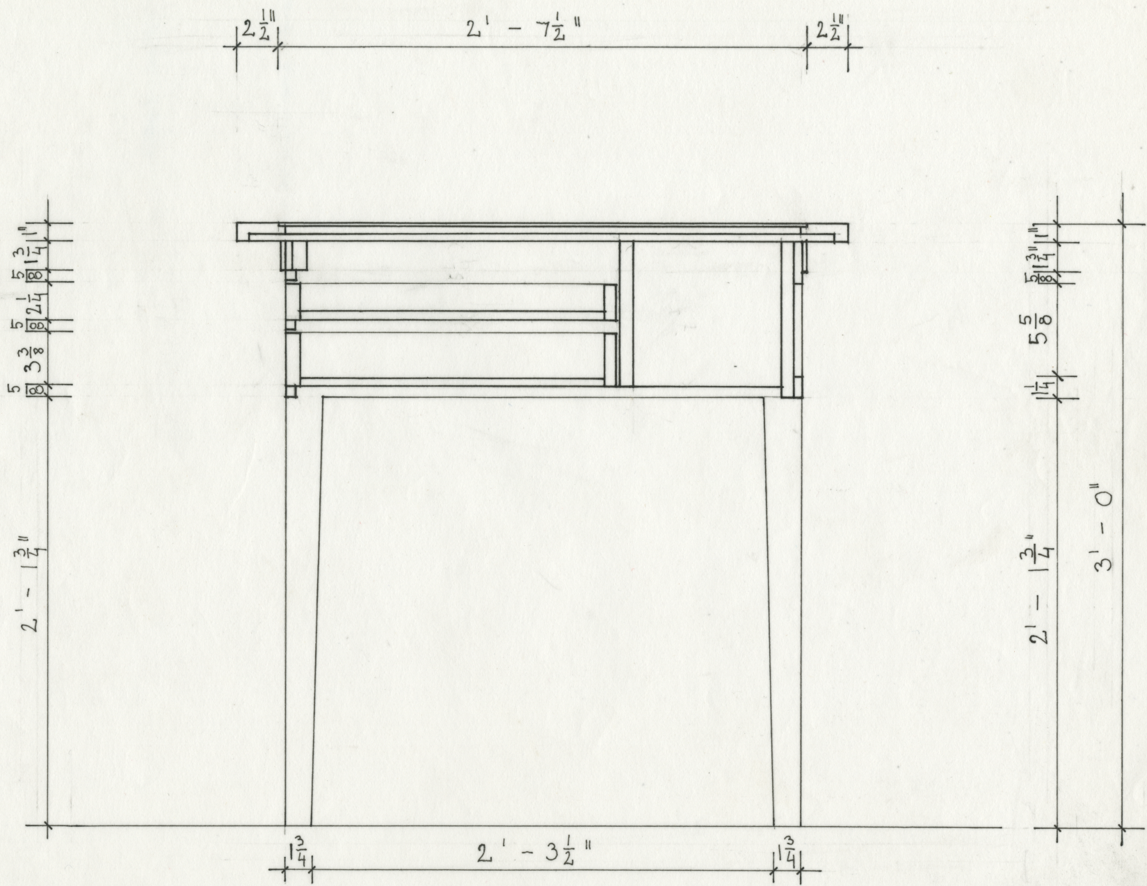
VERTICAL SECTION \frac{1}{2}'' = 1'-0''
