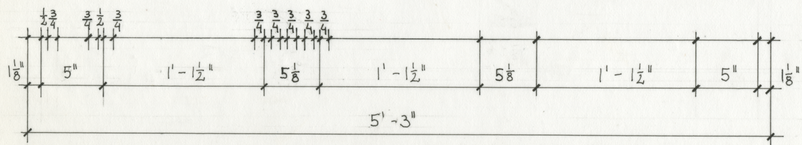
HORIZONTAL SECTION \frac{1}{2}'' = 1' - 0''
