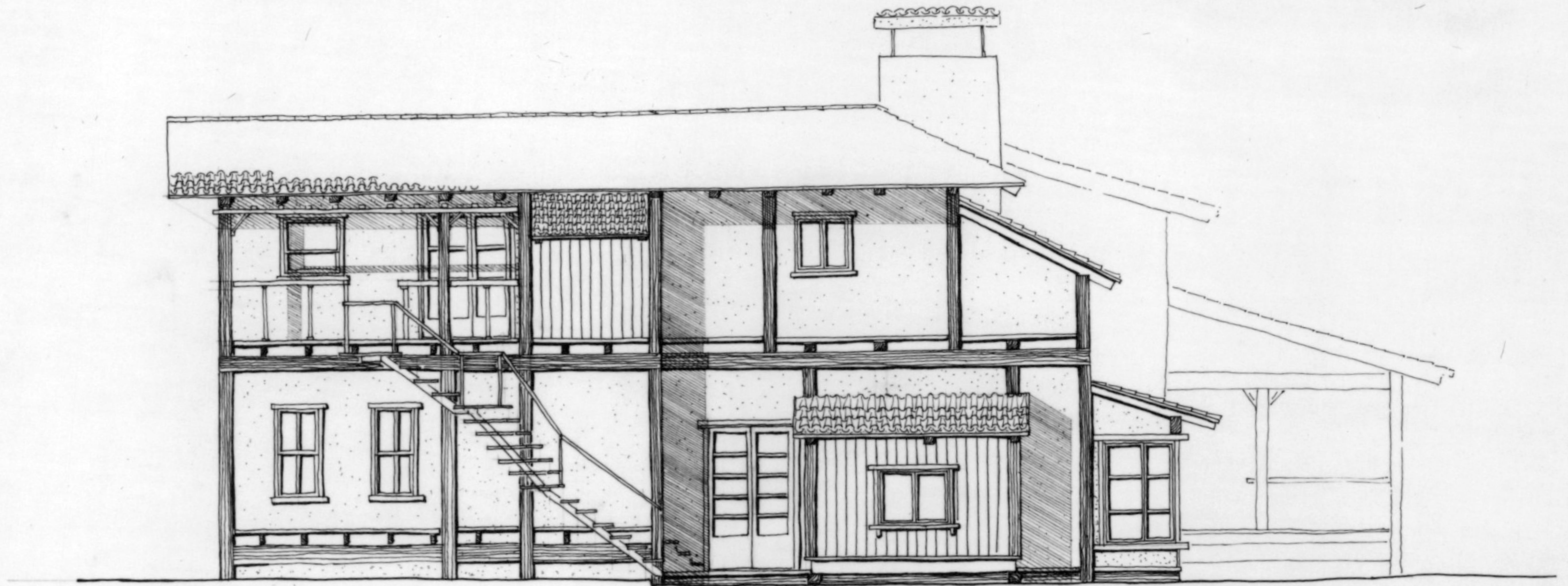
WEST ELEVATION
