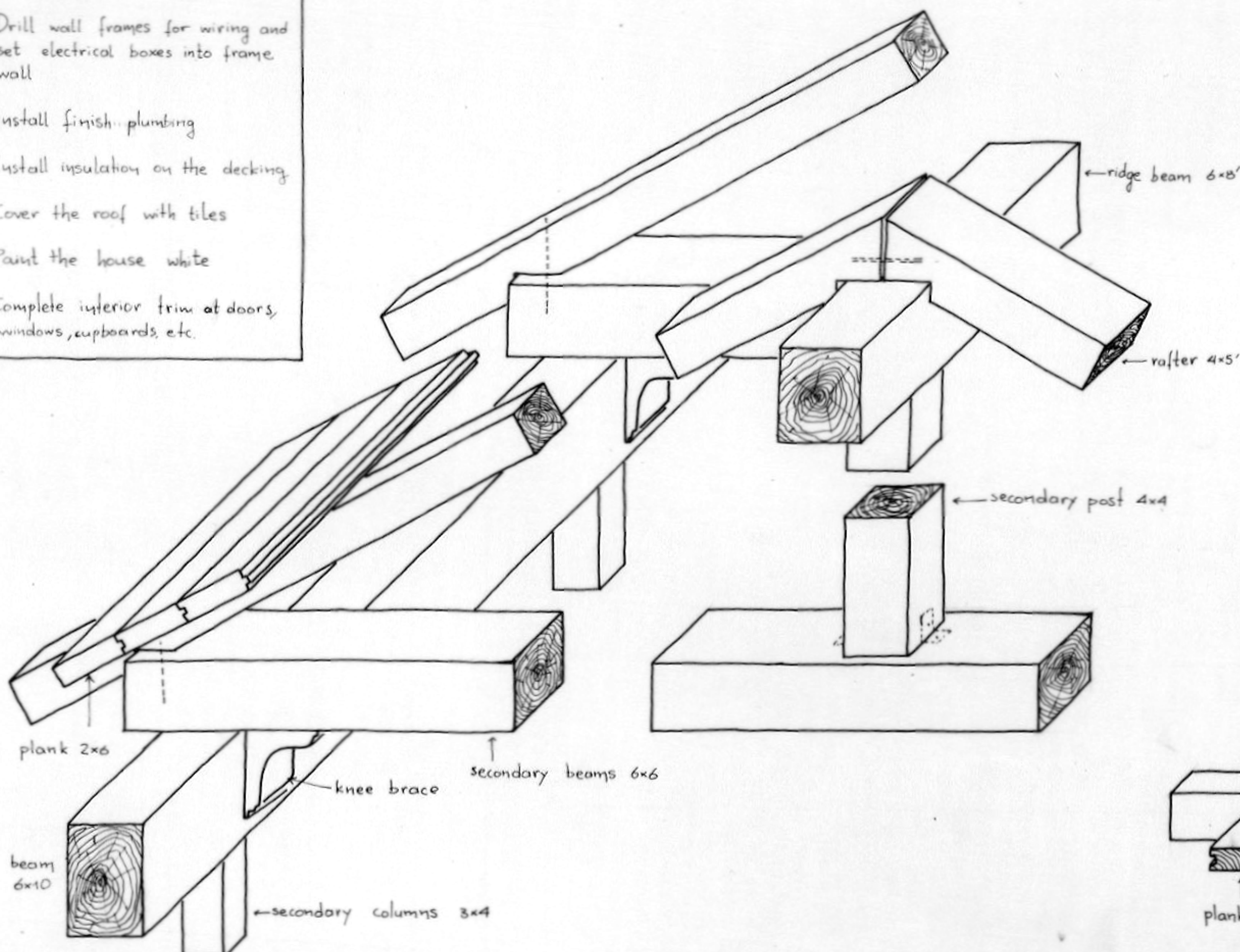
ROOF FRAMING CONSTRUCTION
