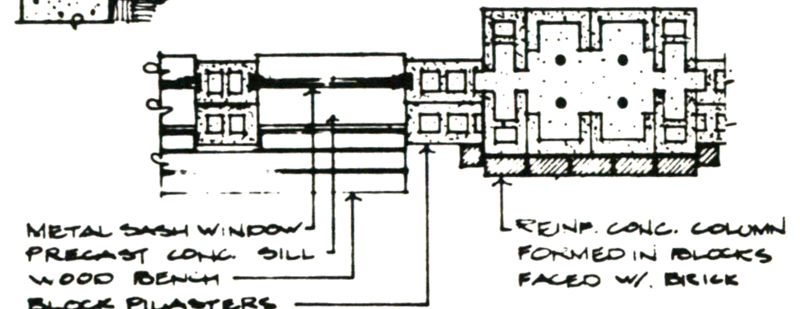
HORIZONTAL SECTION: NORTHEAST WALL
