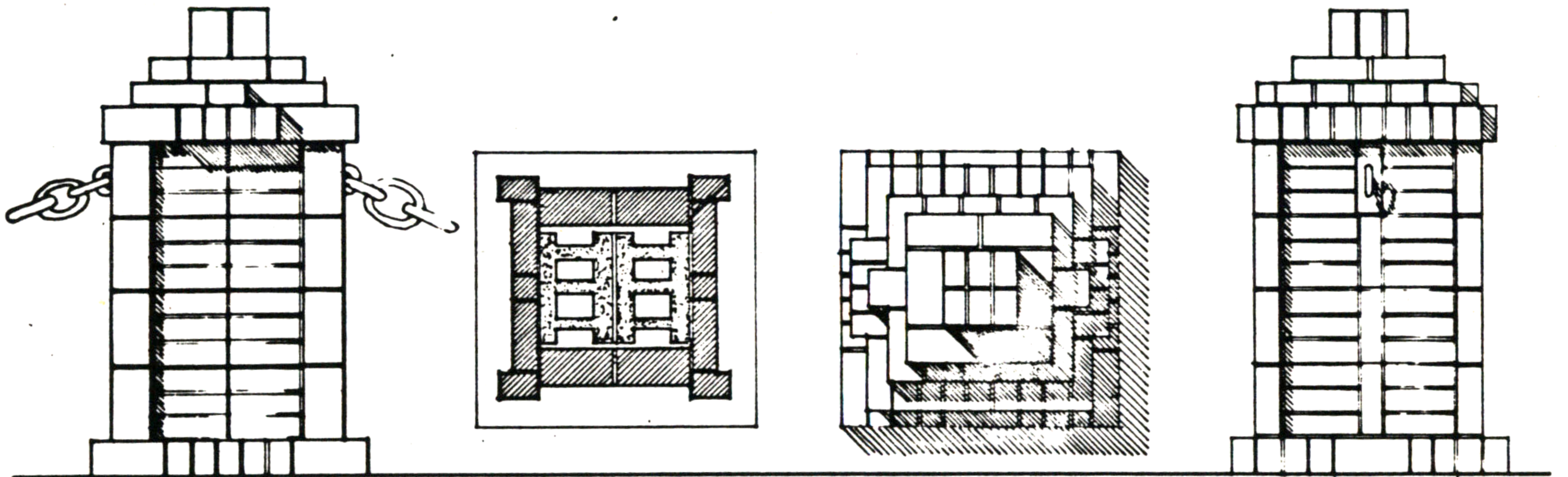
HORIZONTAL SECTION
