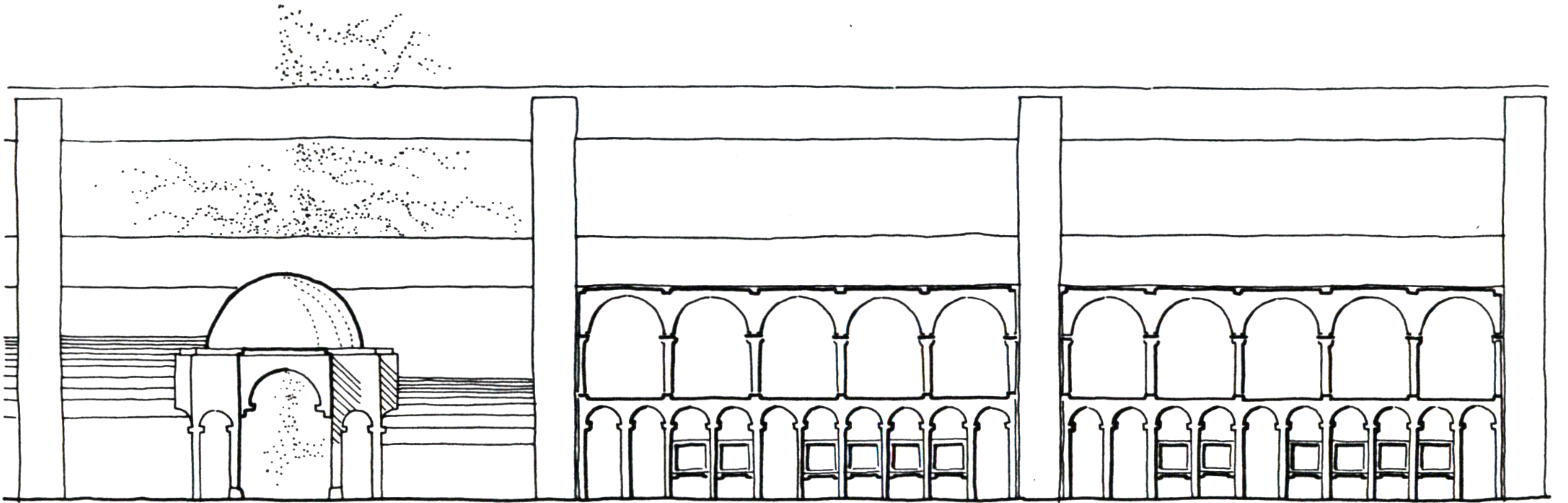
SOUTH WEST ELEVATION
