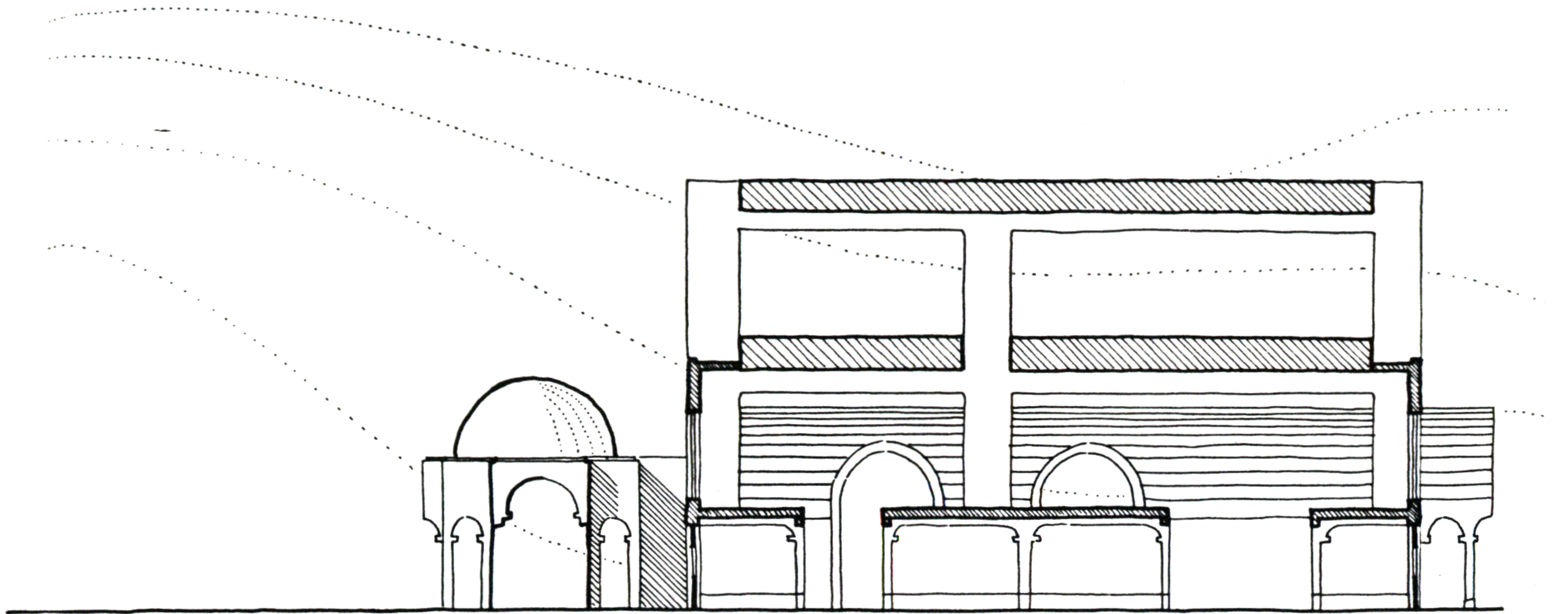
SECTION AA
