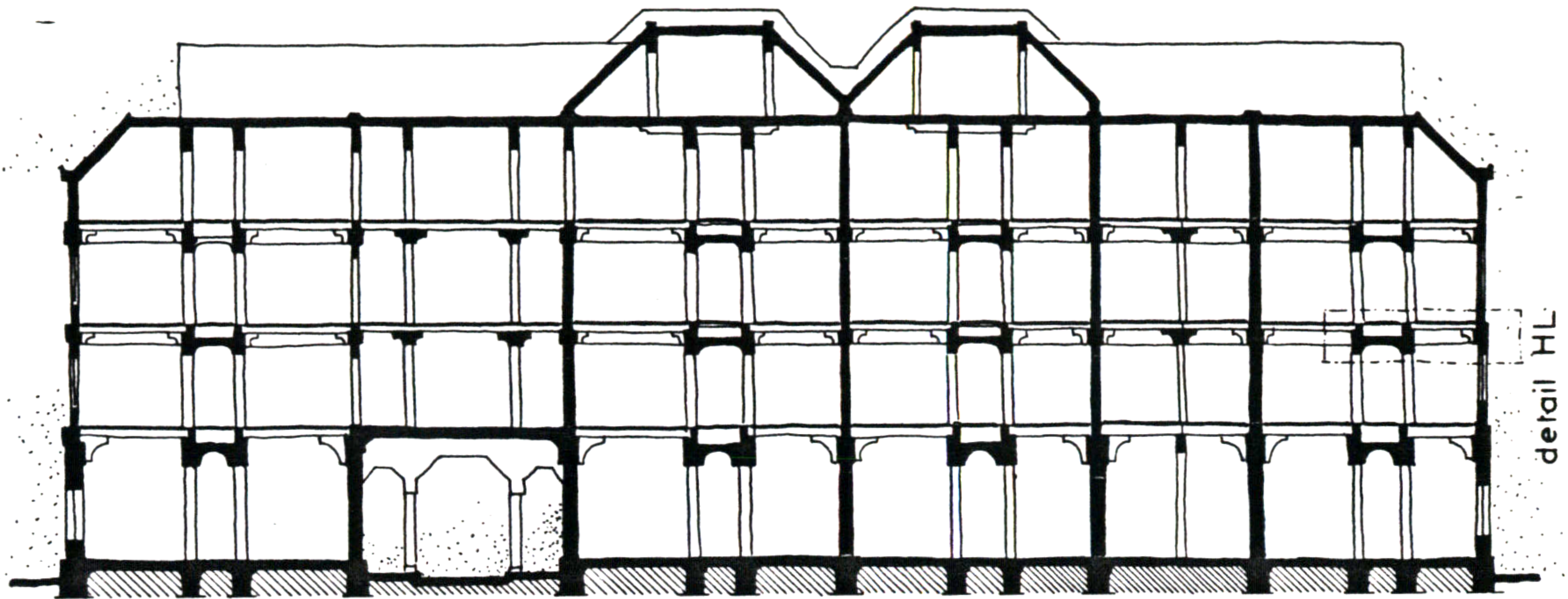
SECTION AA
