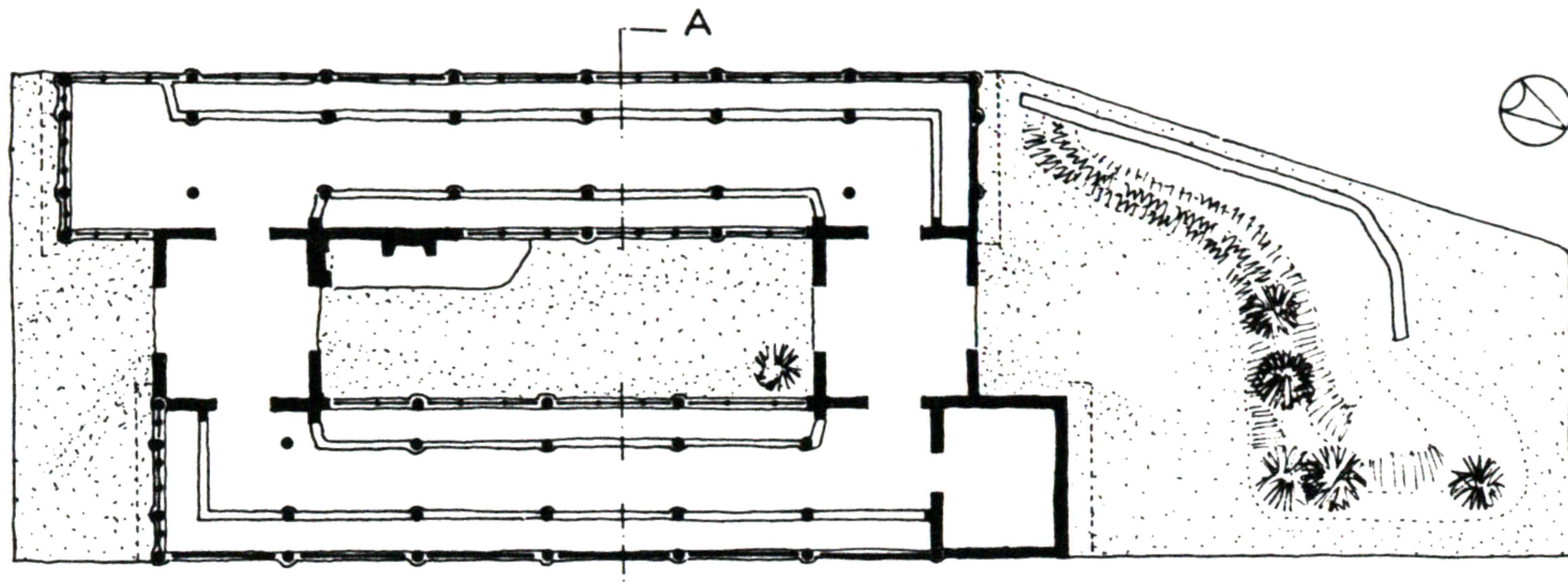
FLOORPLAN
