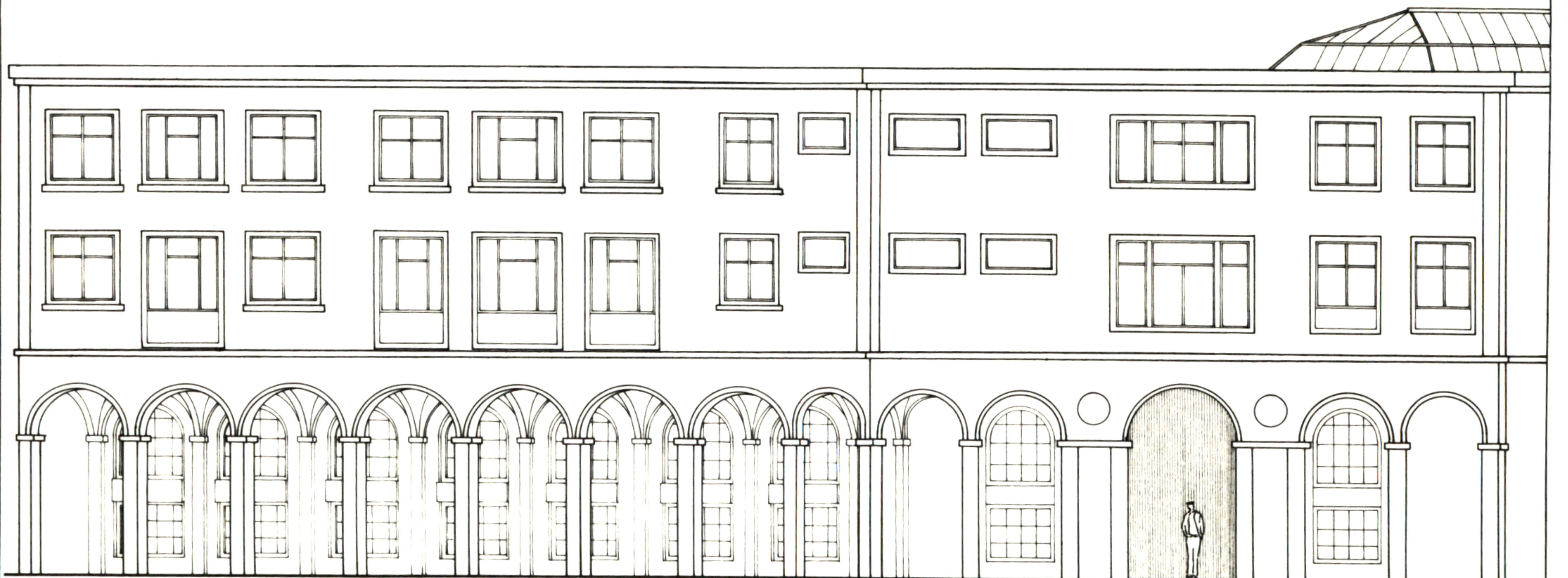
SOUTH -WEST ELEVATION ON THE STREET
