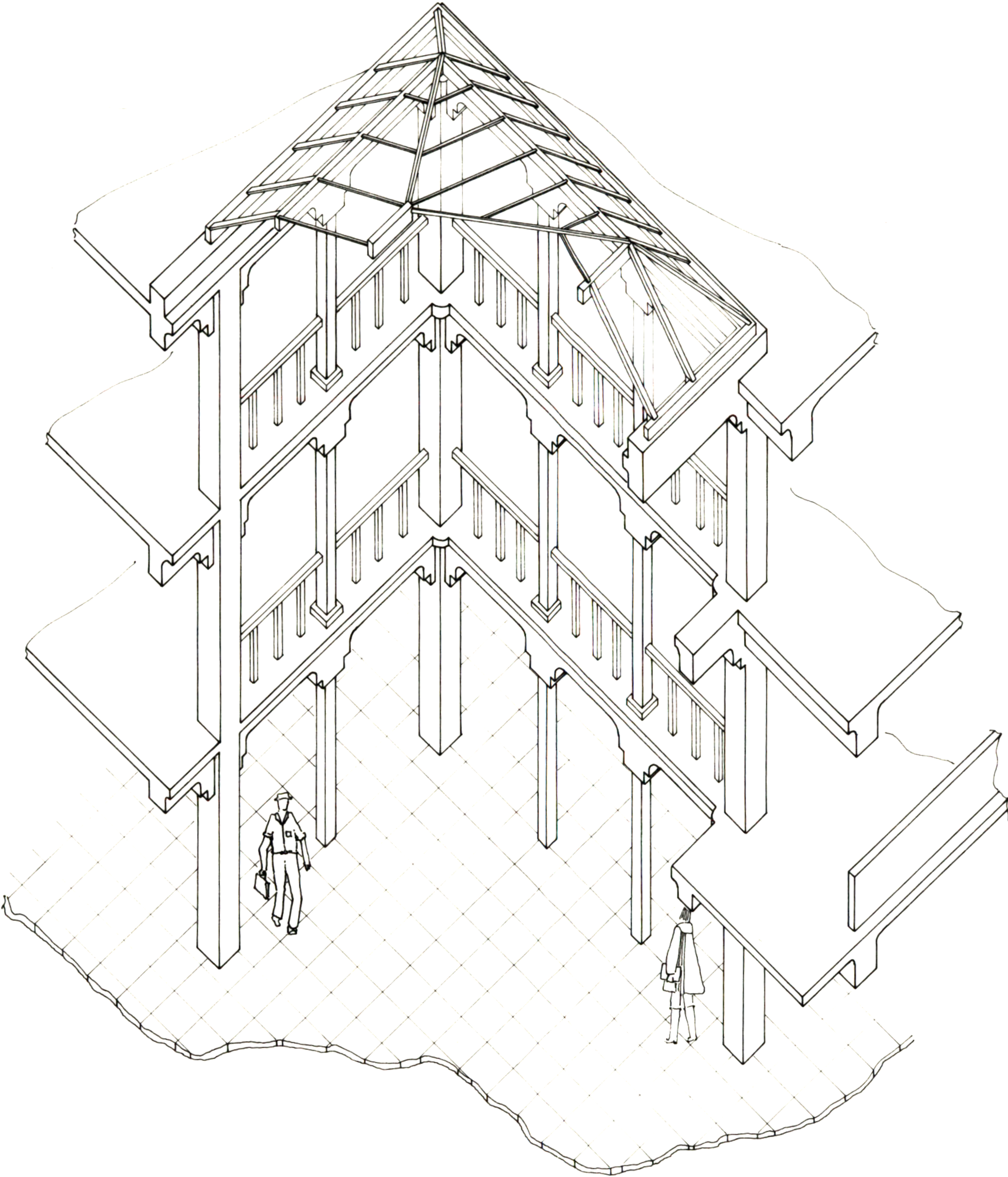
AXONOMETRIC OF THE LOBBY
