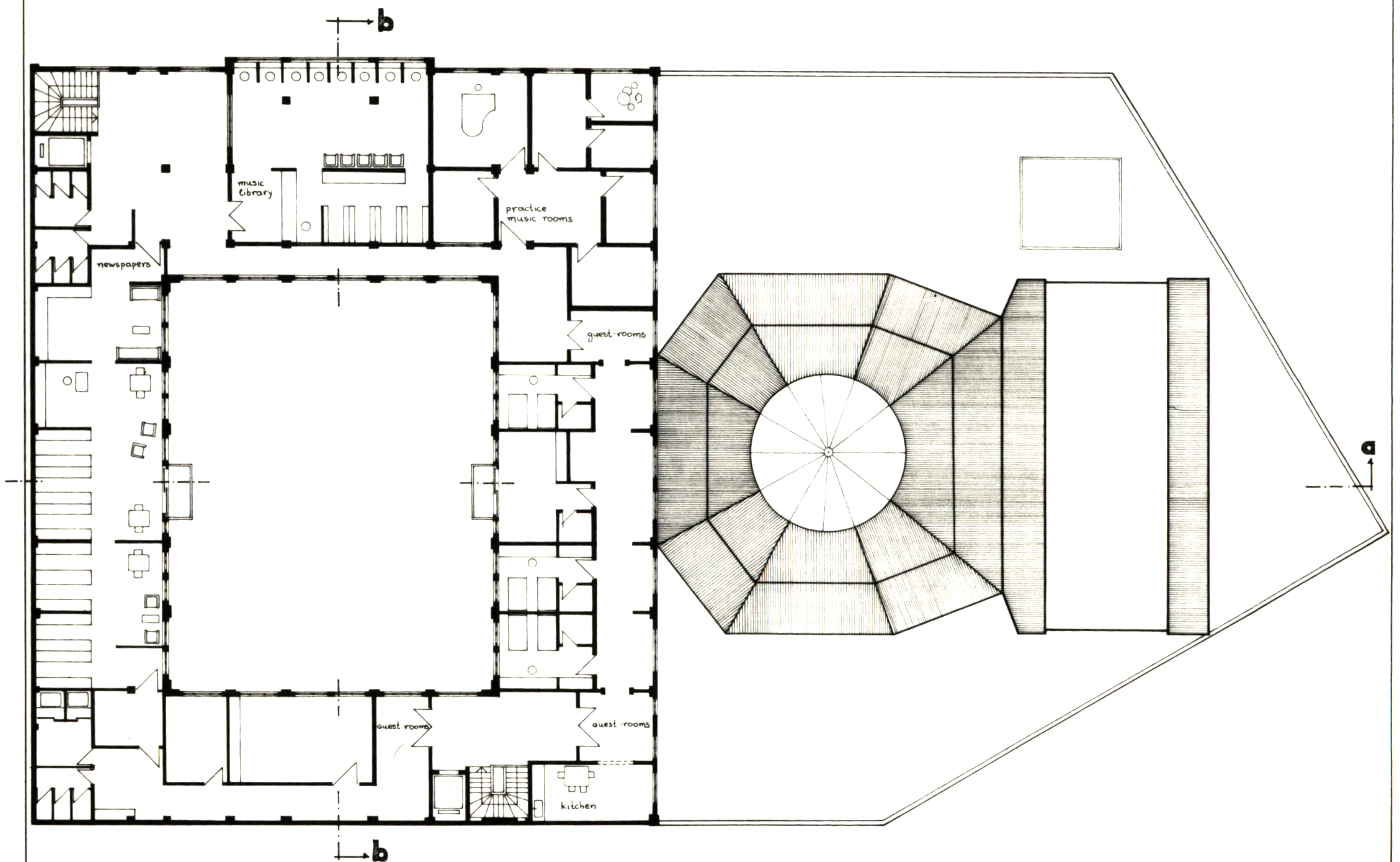
FIFTH FLOOR PLAN
