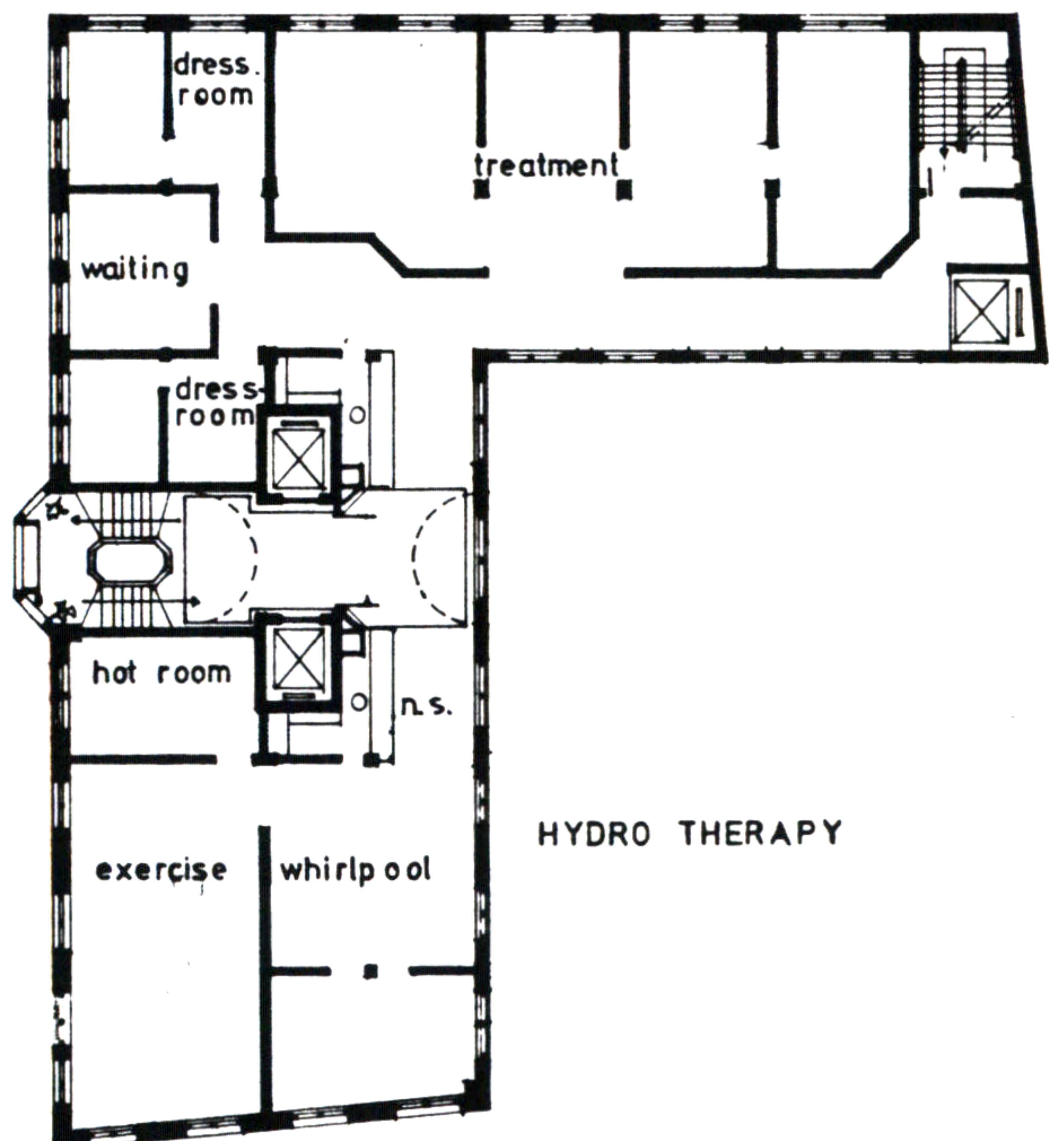
SIXTH FLOOR PLAN
