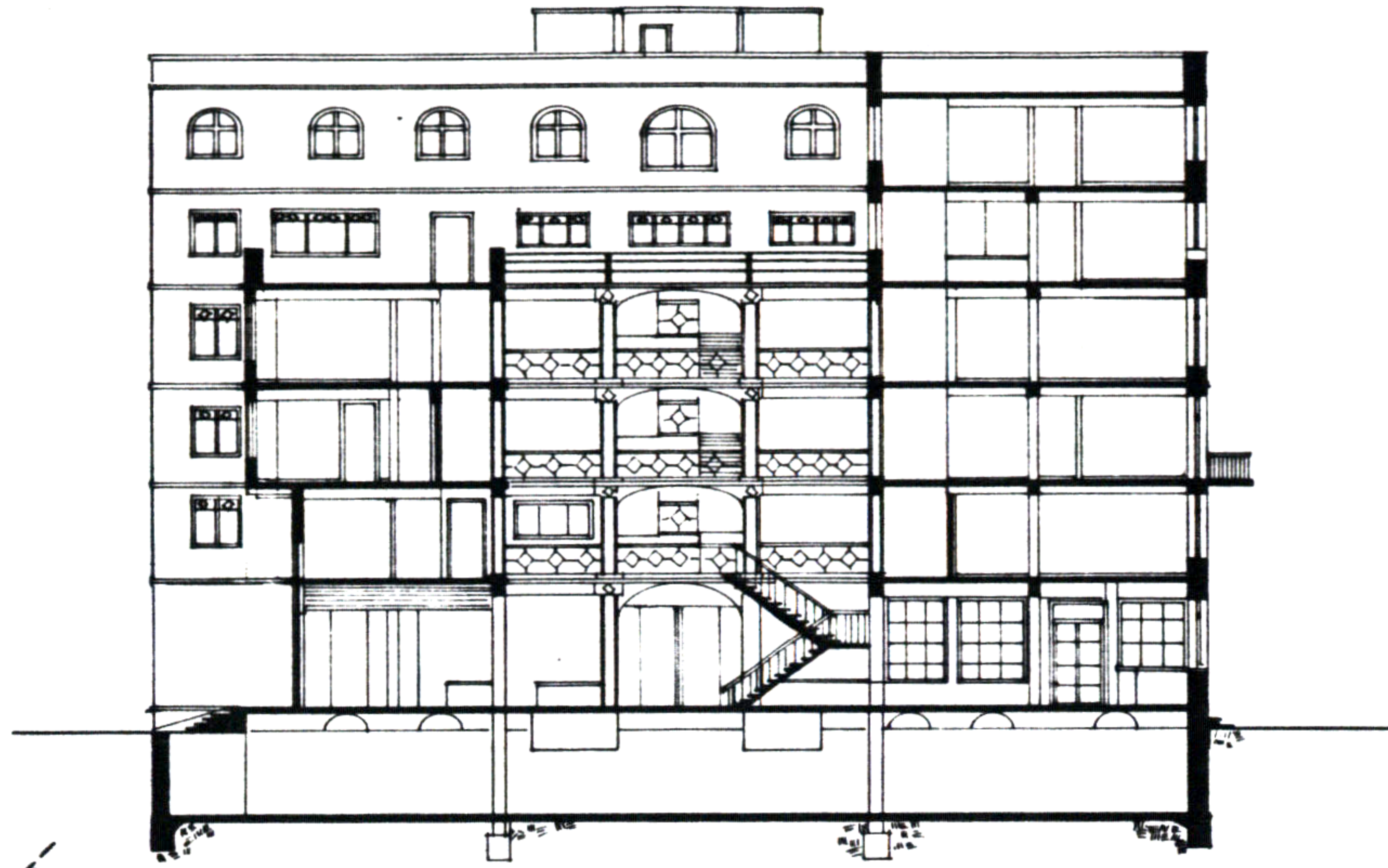
SECTION B-B
