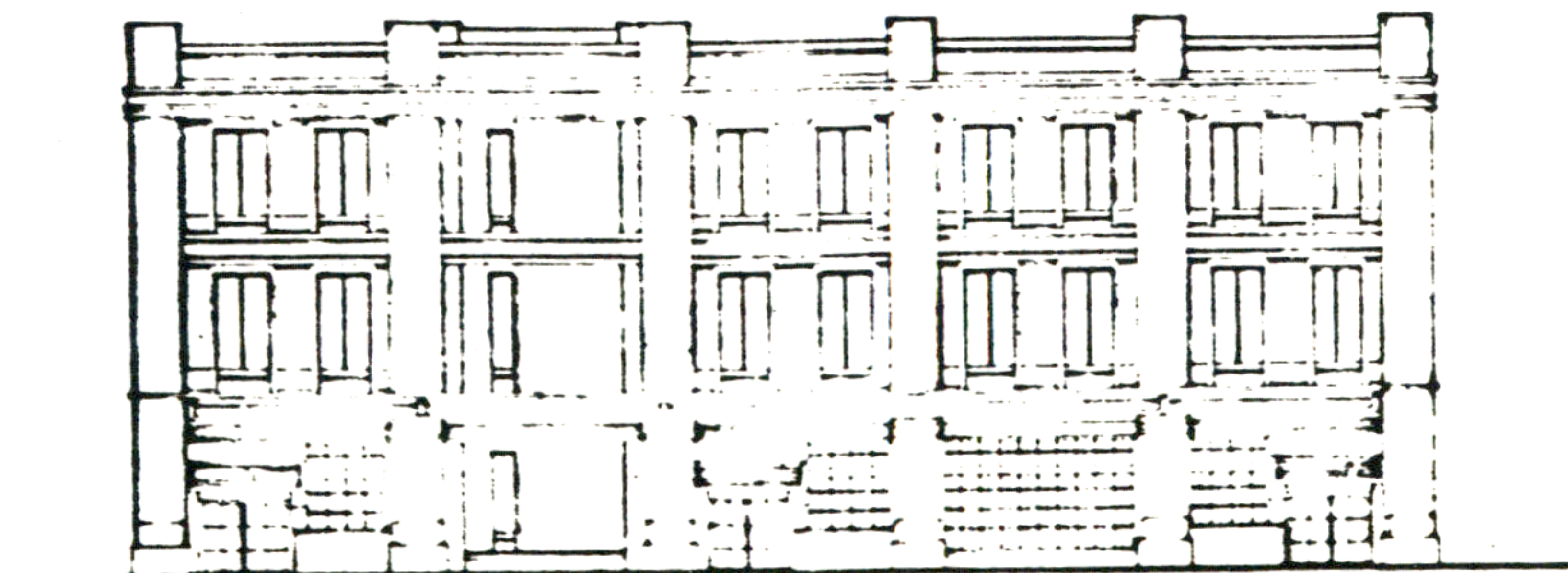
EAST ELEVATION
