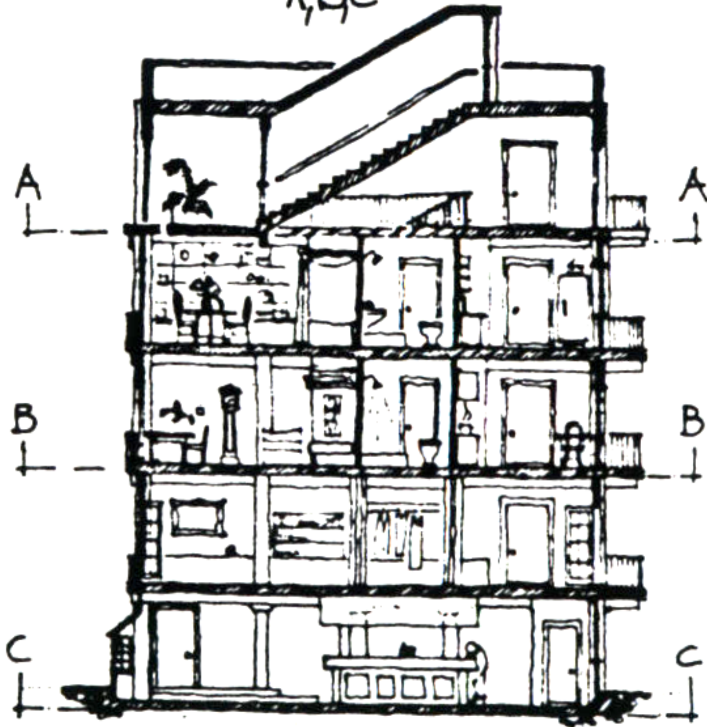
SECTION A/B/C
