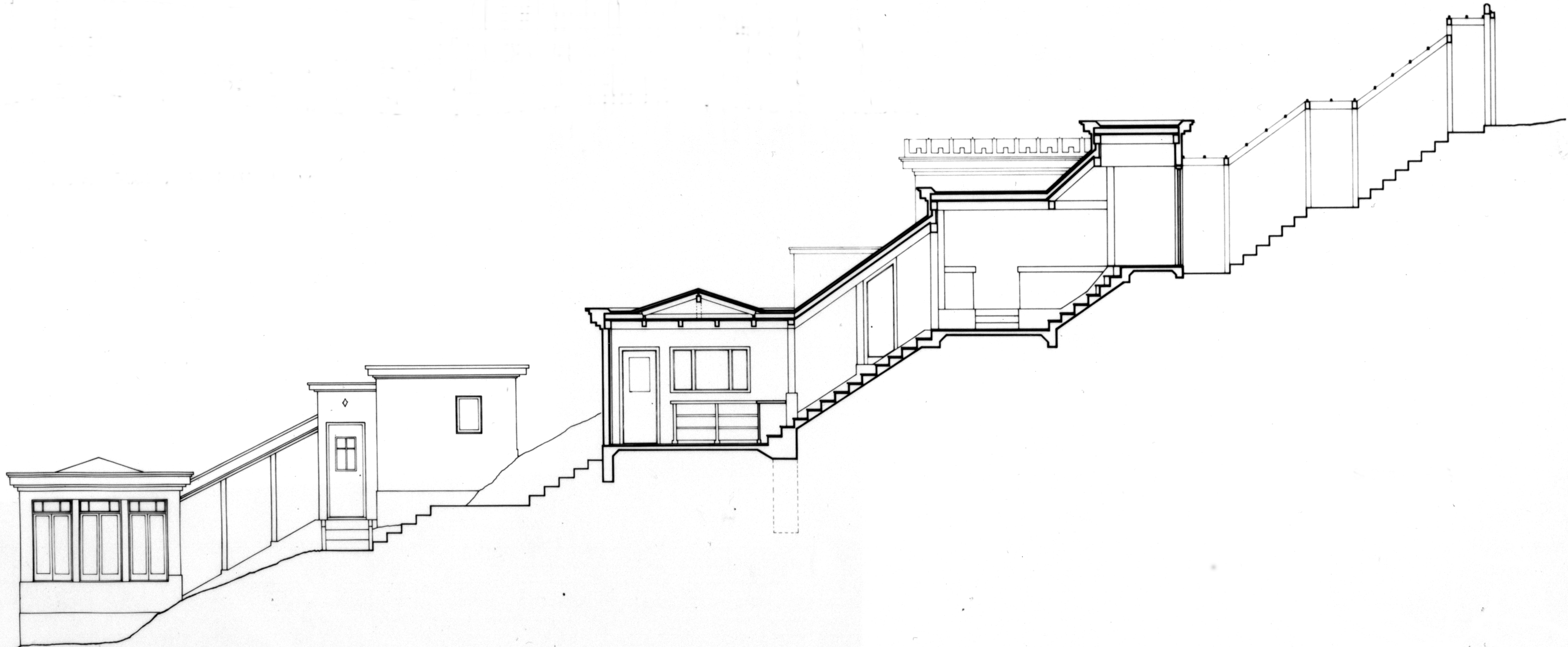
LIBRARY-BEDROOM ELEVATION south-west
