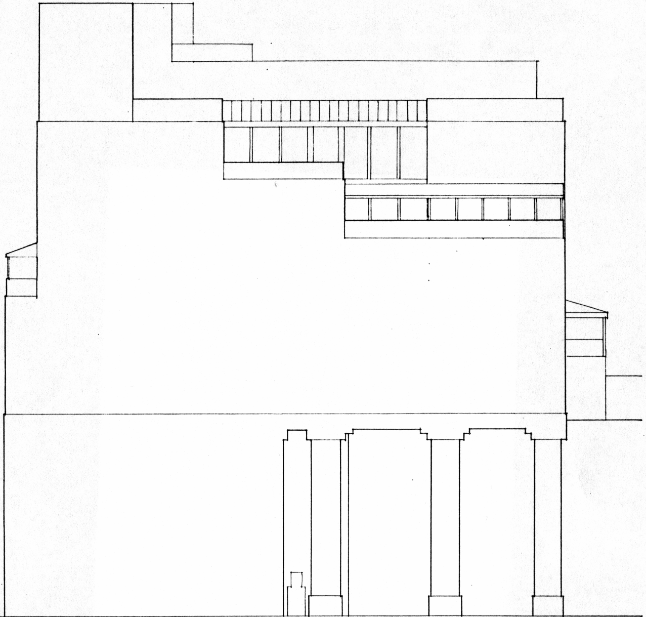
east elevation
