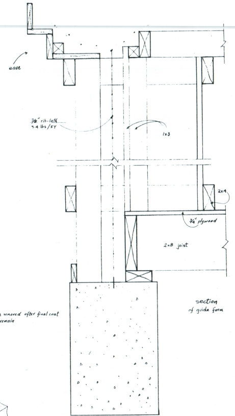
Corner Column Details scale: 1/4 page 6 of 8
