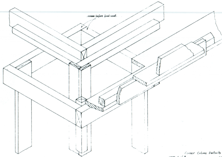
Corner Column Details scale: 1/4 page 6 of 8
