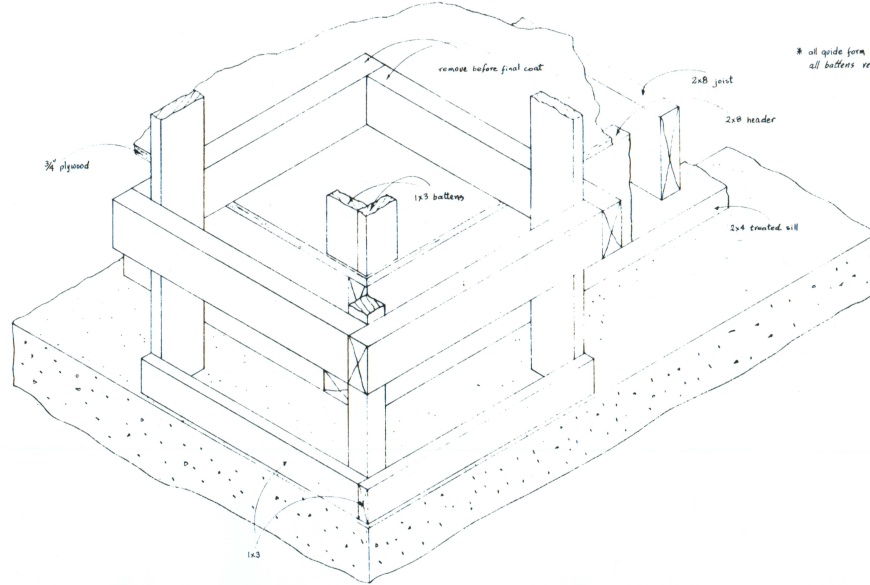
Corner Column Details scale: 1/4 page 6 of 8
