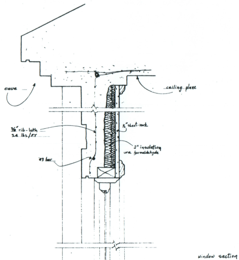
Window section
