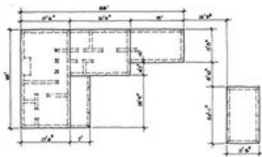
FOUNDATION PLAN 1" = 10'-0"
