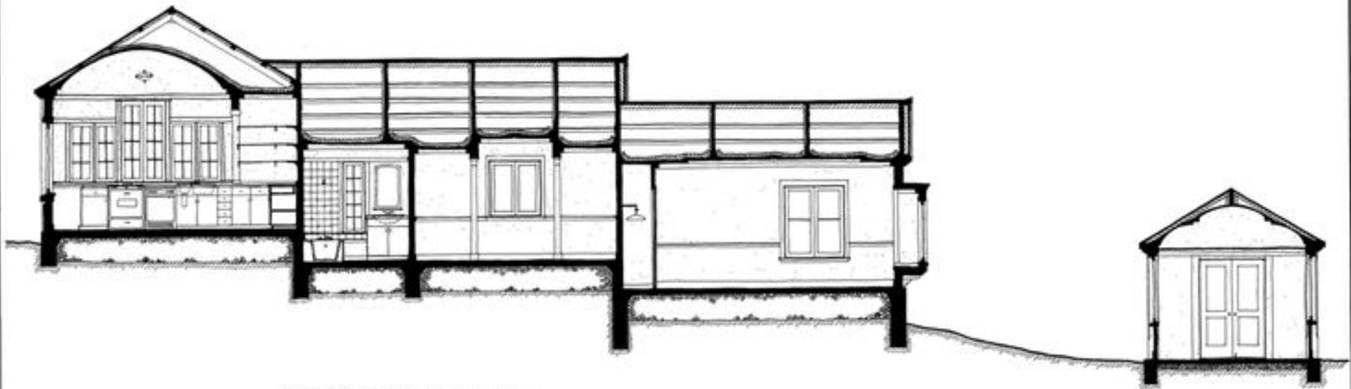
BUILDING SECTION (LOOKING SOUTHWEST) 1/8" = 1'-0"
