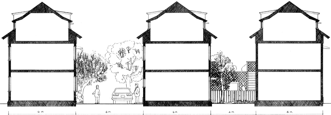
TYPICAL CROSS SECTION. SCALE 1:50
