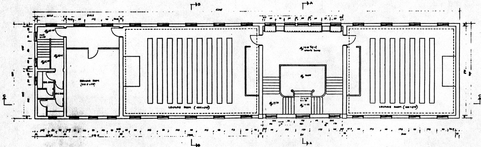
SECOND FLOOR PLAN 1/80
