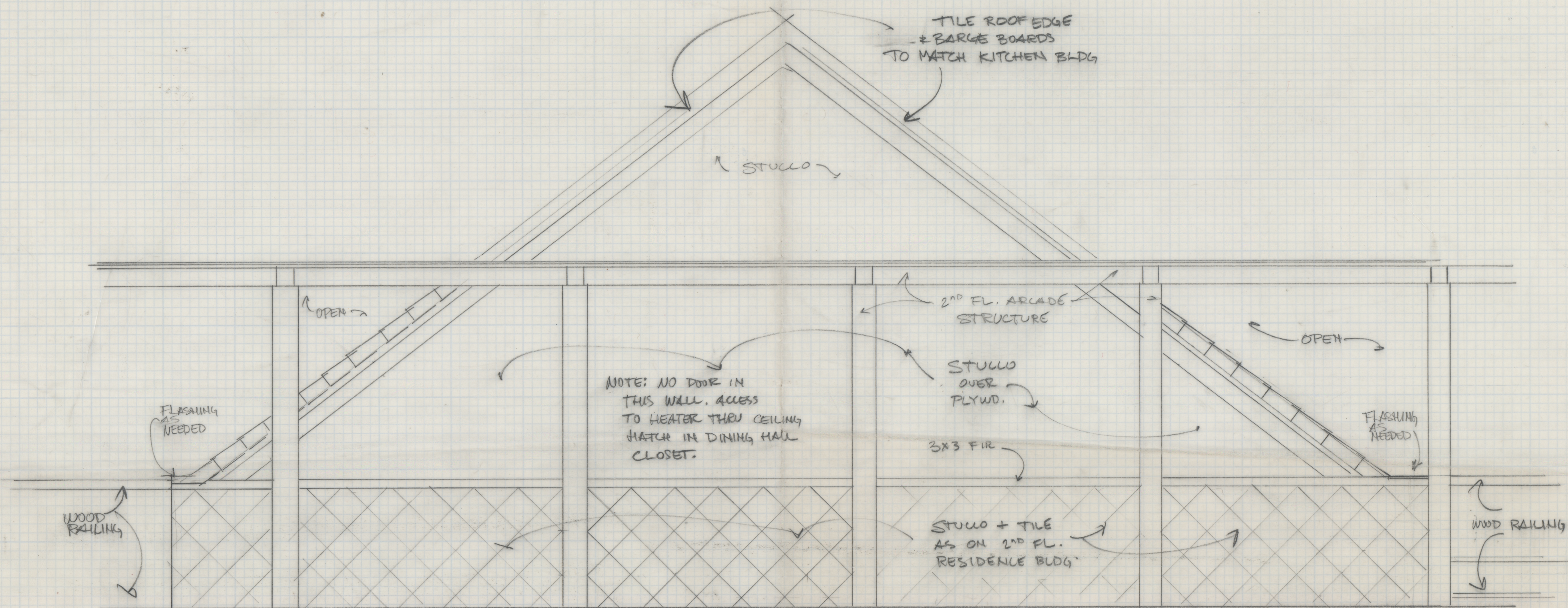
ELEVATION DINING HALL GABLE END @ 2ND FLOOR ARCADE
