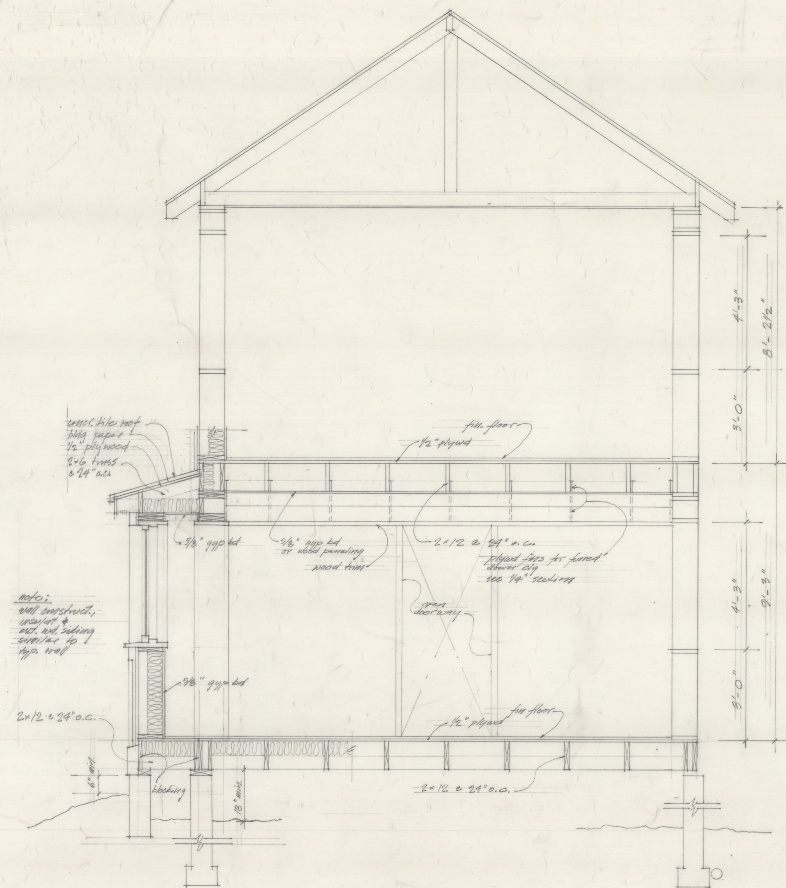
SECTION B-B KITCHEN/DINING ROOM 1/2" = 1'-0"
