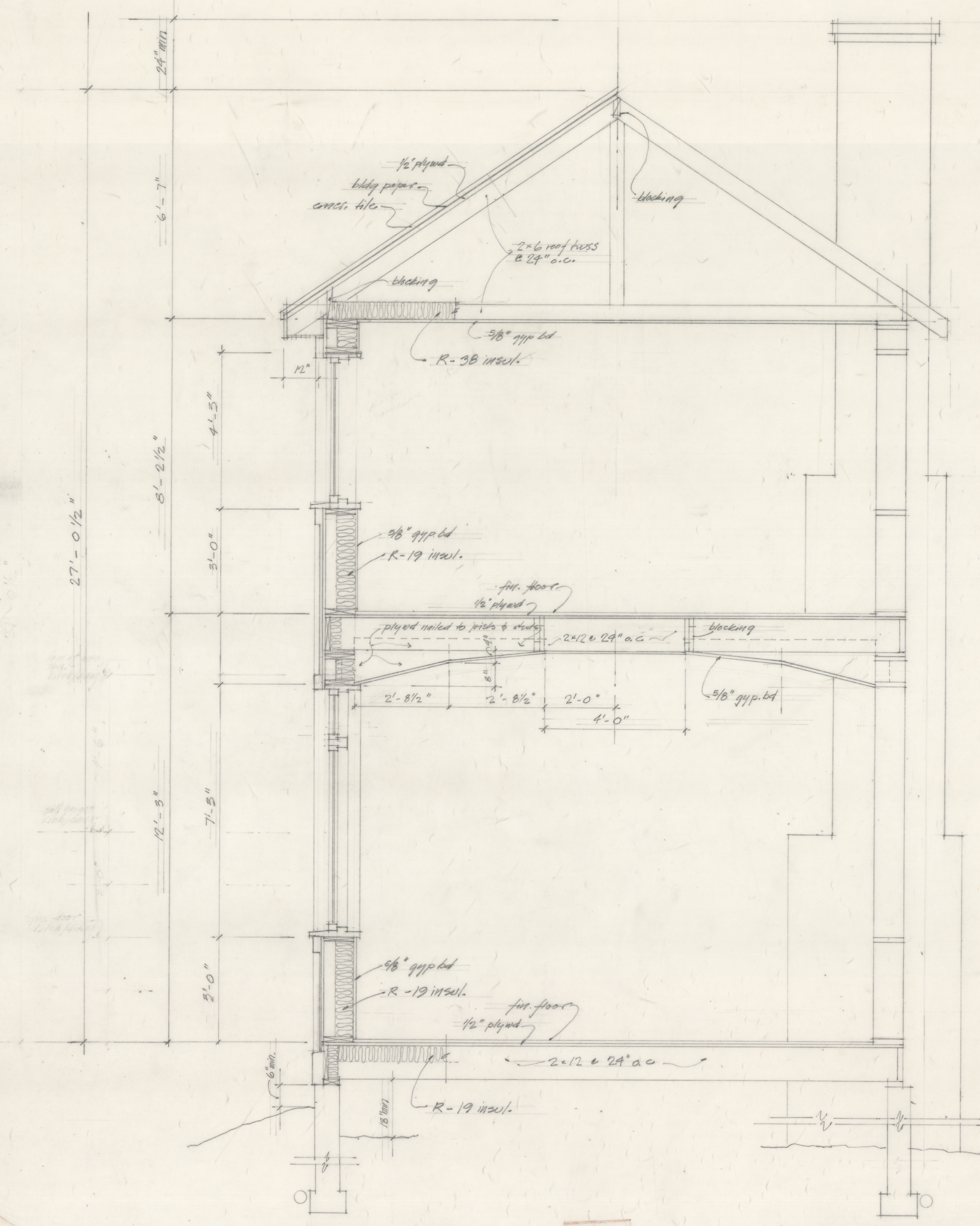
SECTION A-A LIVING ROOM 1/2" = 1'-0"
